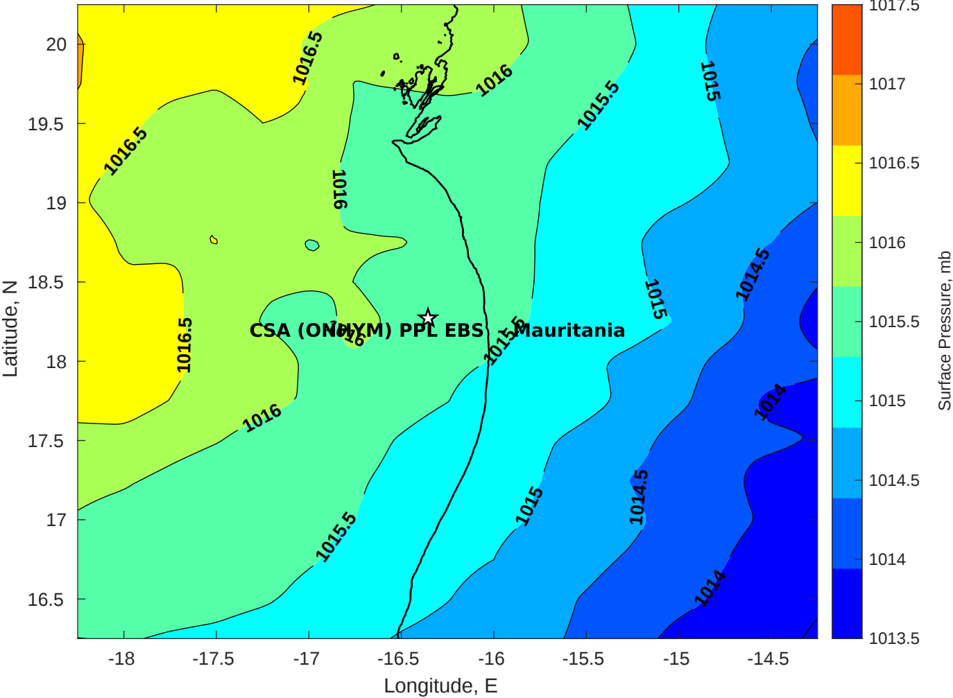
Surface Pressure (mb) for CSA (ONHYM) PPL EBS - Mauritania at 14-Dec-2025 00:00:00
