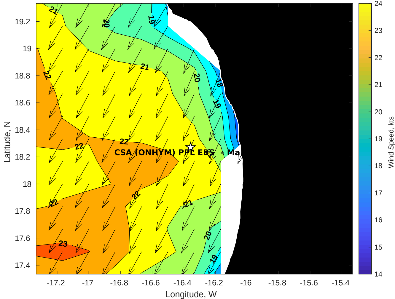
GFS Winds (kts) for CSA (ONHYM) PPL EBS - Mauritania at 13-Dec-2025 09:00:00
