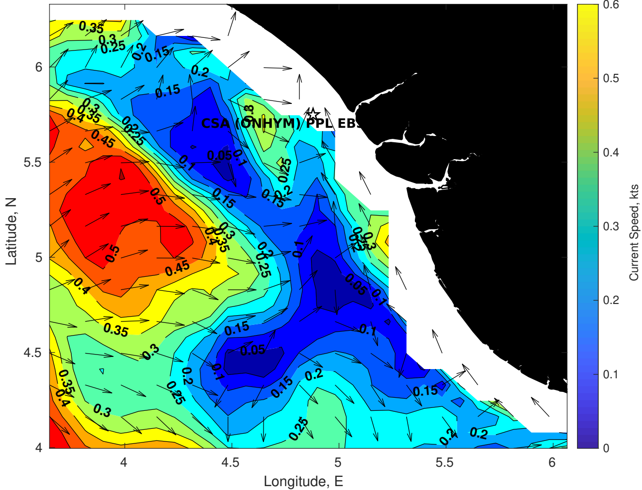
Surface Currents for CSA (ONHYM) PPL EBS - Nigeria at 12-Dec-2025 00:00:00
