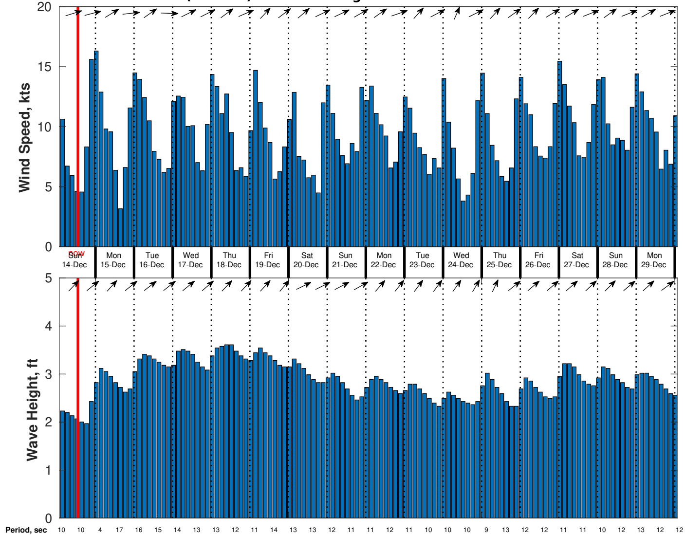
Wind & Wave Forecast for CSA (ONHYM) PPL EBS - Nigeria from 13-Dec-2025 02:00:00 to 29-Dec-2025 02:00:00
