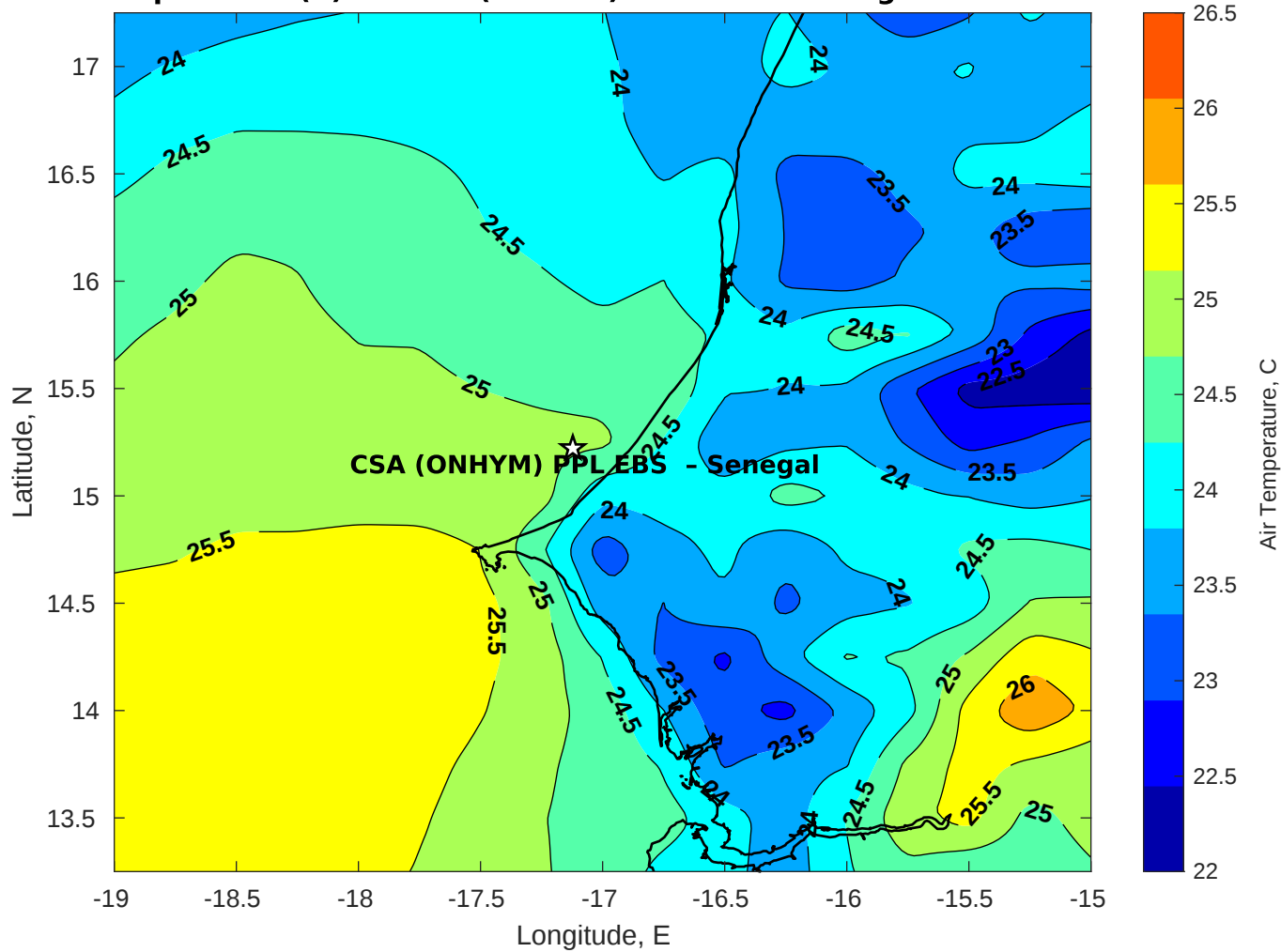
Air Temperature (C) for CSA (ONHYM) PPL EBS - Senegal at 13-Dec-2025
