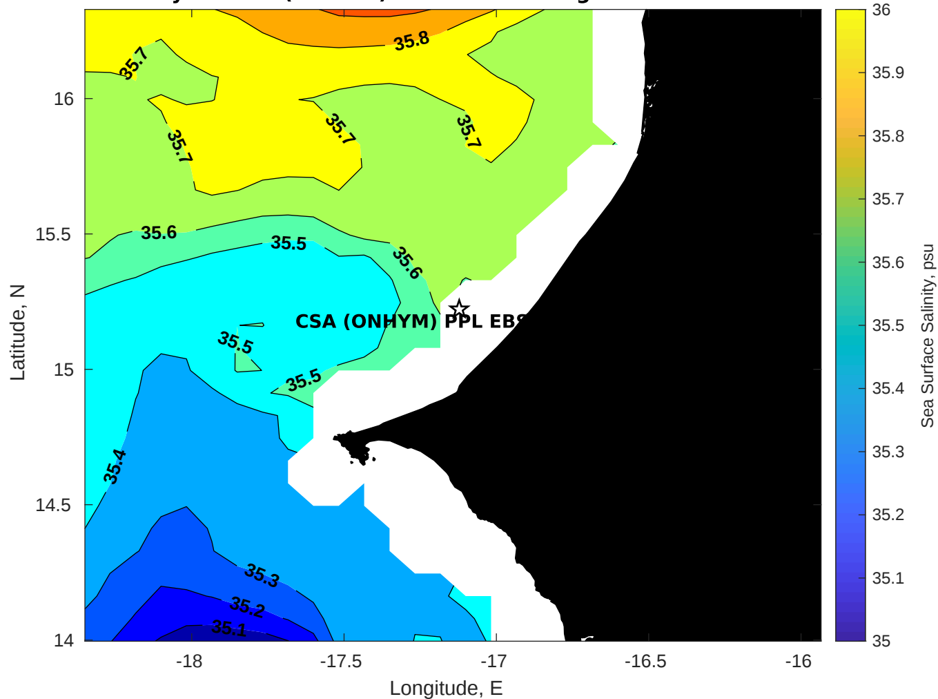
Surface Salinity for CSA (ONHYM) PPL EBS - Senegal at 12-Dec-2025 00:00:00
