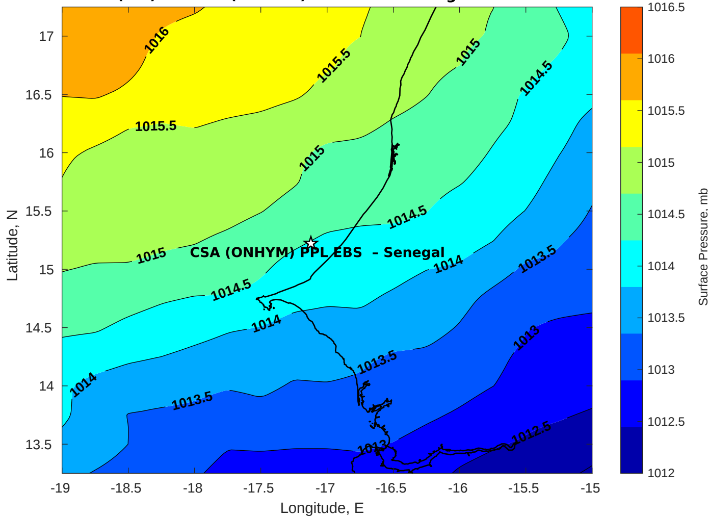
Surface Pressure (mb) for CSA (ONHYM) PPL EBS - Senegal at 14-Dec-2025 00:00:00
