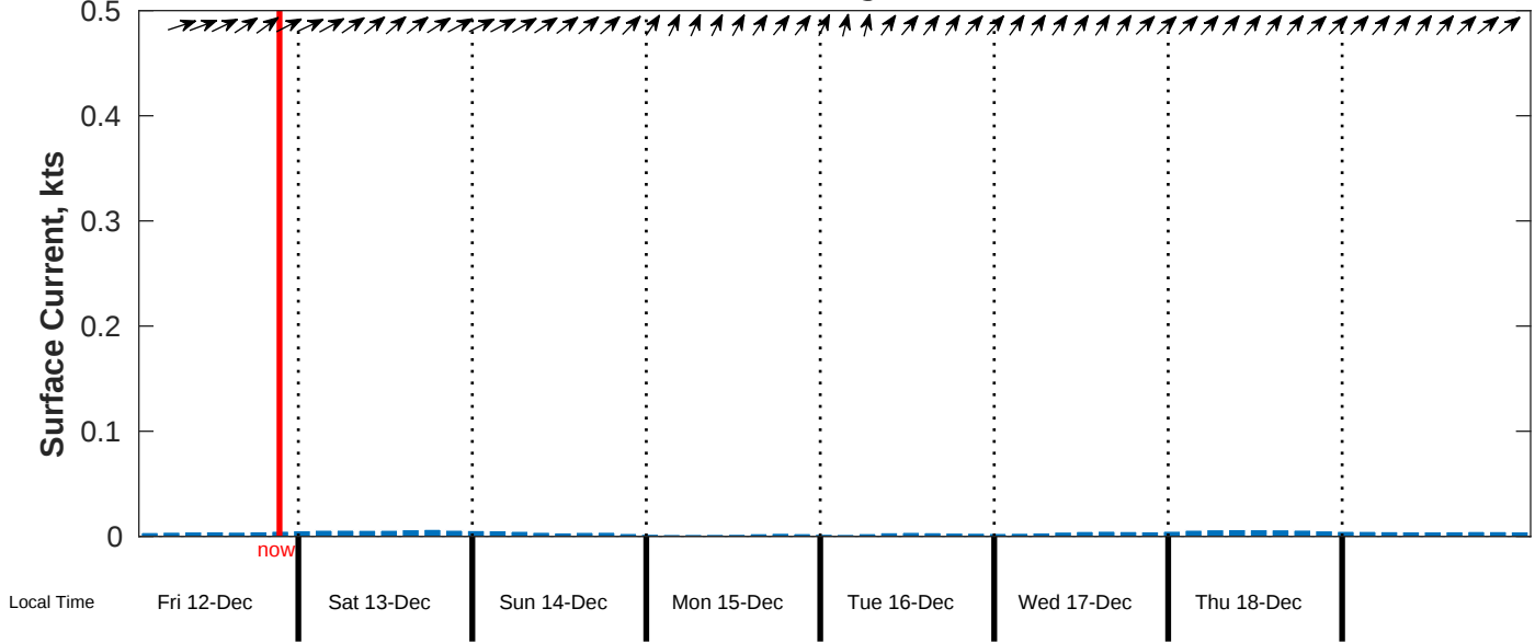
Surface Current Forecast for CSA (ONHYM) PPL EBS - Senegal from 12-Dec-2025 00:00:00 to 20-Dec-2025 00:00:00
