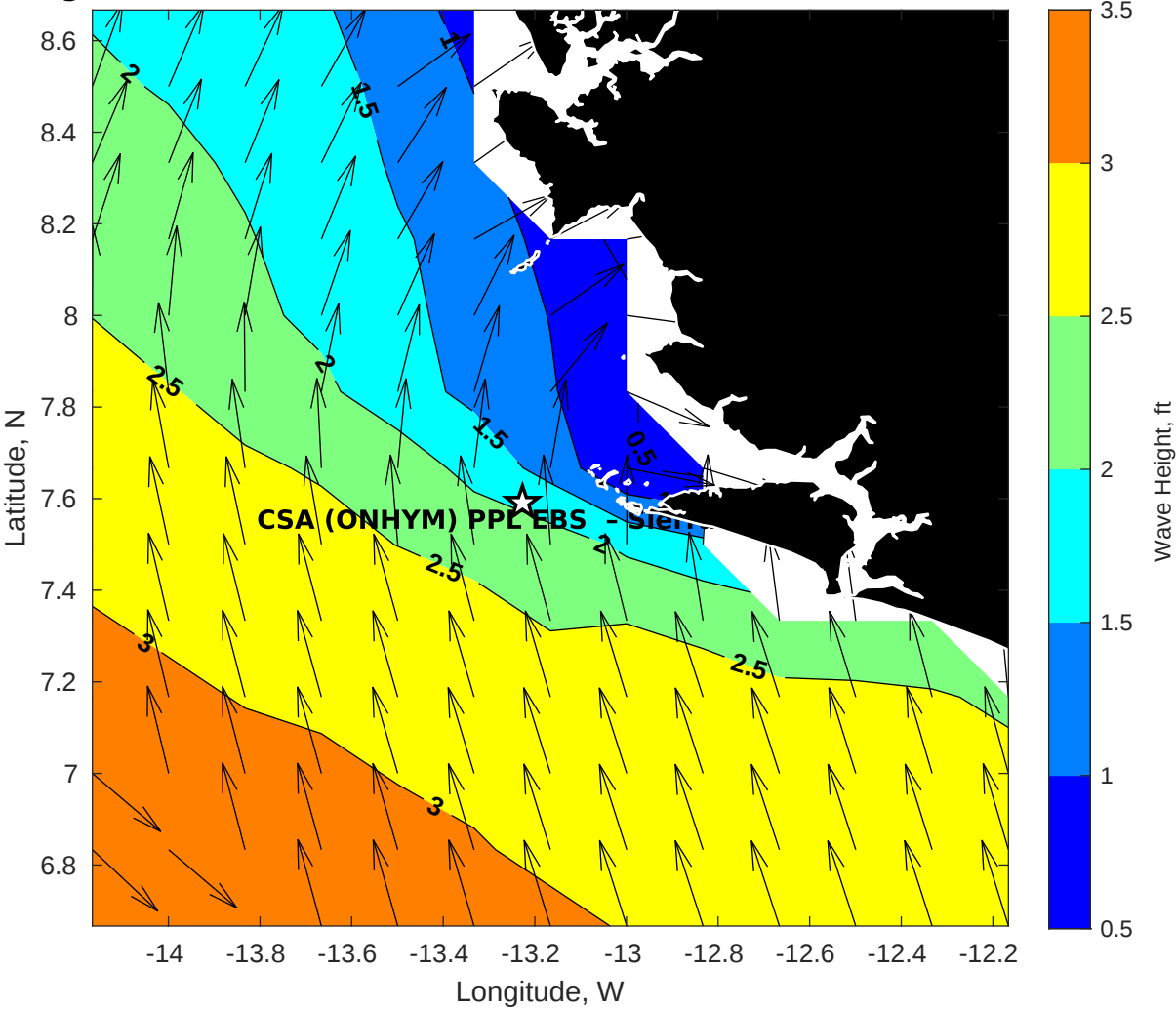
GFS Wave Height (ft) for CSA (ONHYM) PPL EBS - Sierra Leone at 13-Dec-2025 09:00:00
