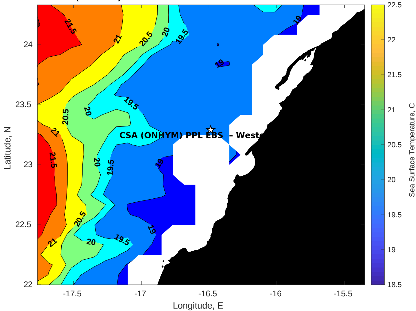
SST for CSA (ONHYM) PPL EBS - Western Sahara at 12-Dec-2025 00:00:00
