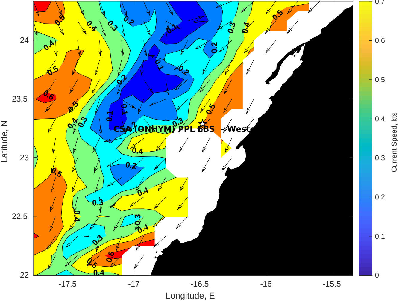
Surface Currents for CSA (ONHYM) PPL EBS - Western Sahara at 12-Dec-2025 00:00:00
