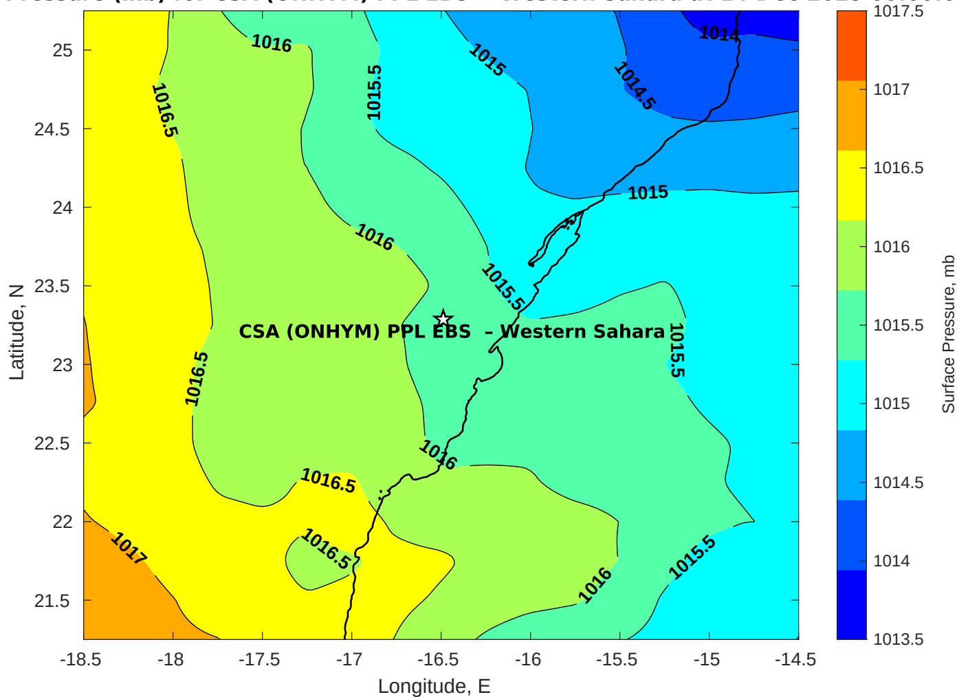
Surface Pressure (mb) for CSA (ONHYM) PPL EBS - Western Sahara at 14-Dec-2025 00:00:00
