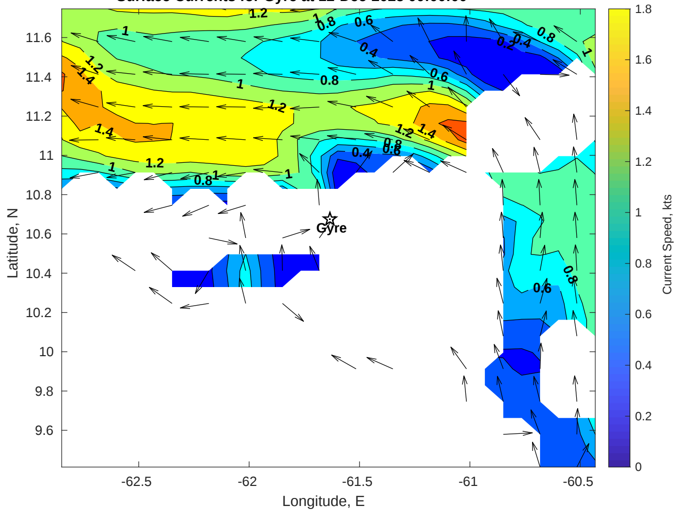
Surface Currents for Gyre at 12-Dec-2025 00:00:00
