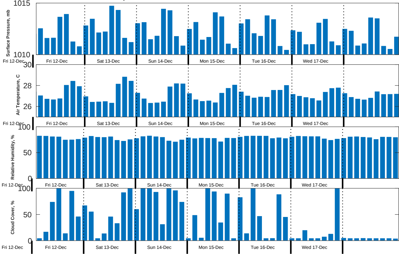
Met Forecast for Gyre from 12-Dec-2025 20:00:00 to 19-Dec-2025 20:00:00
