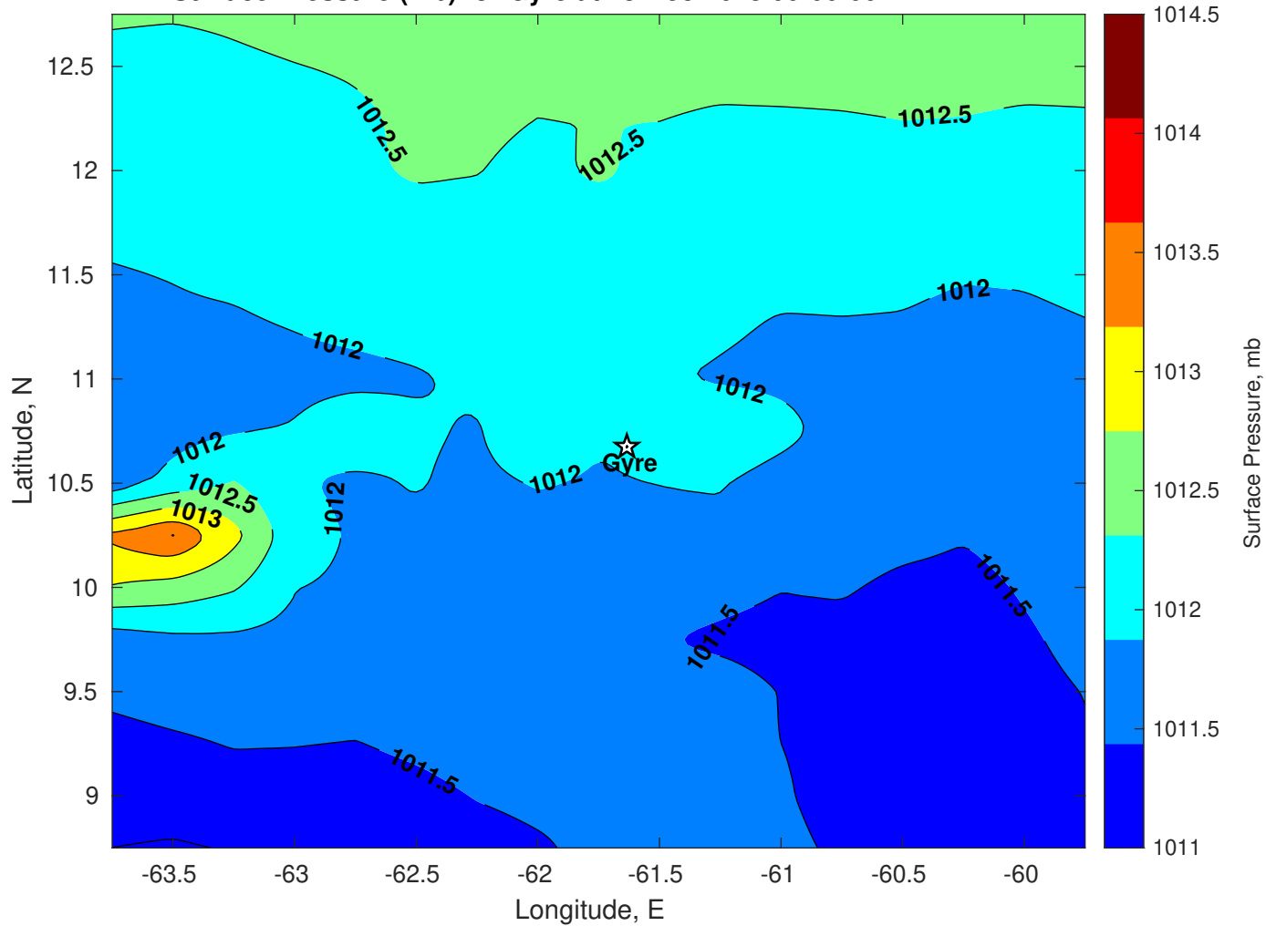
Surface Pressure (mb) for Gyre at 13-Dec-2025 00:00:00
