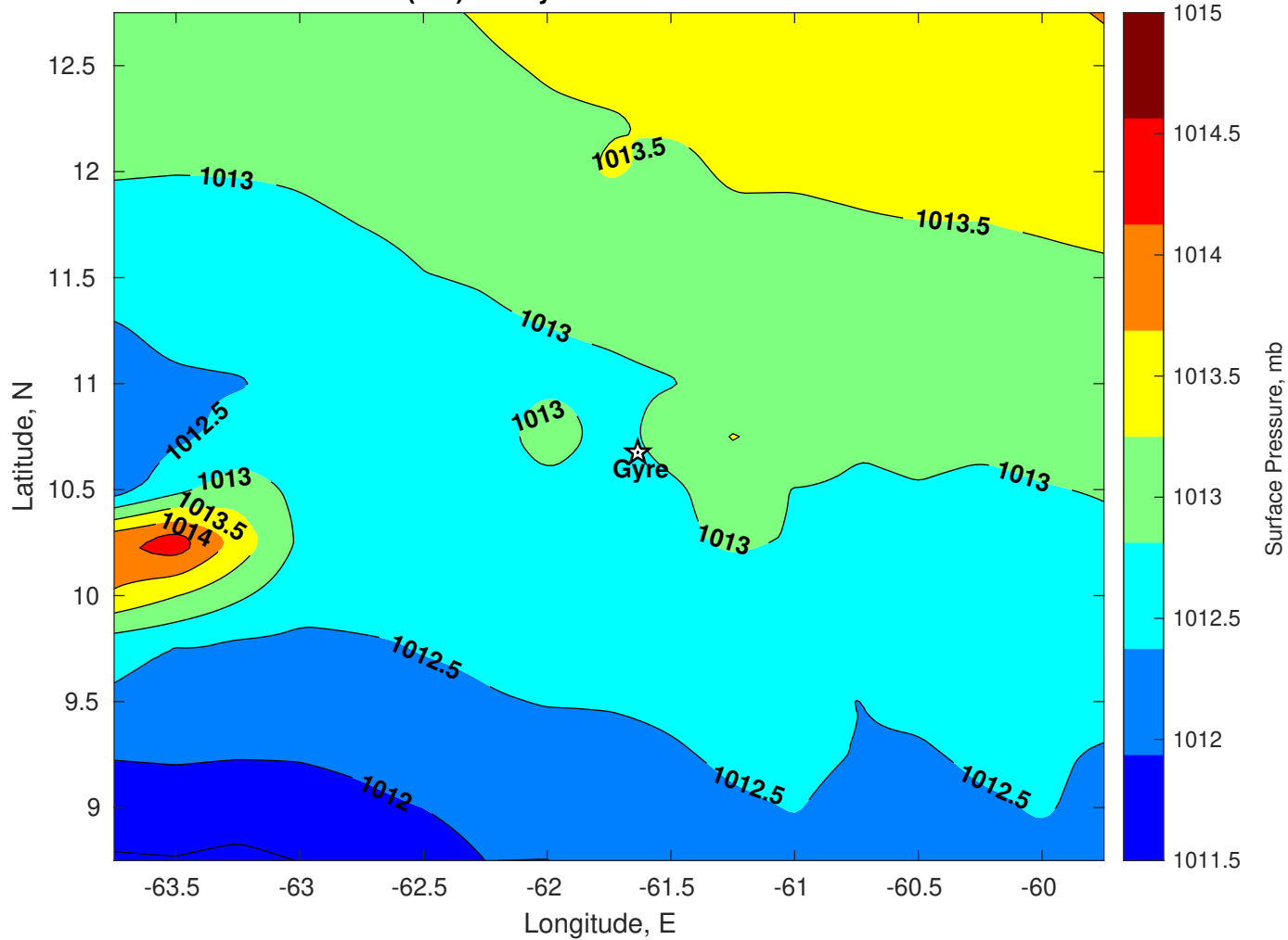
Surface Pressure (mb) for Gyre at 14-Dec-2025 00:00:00
