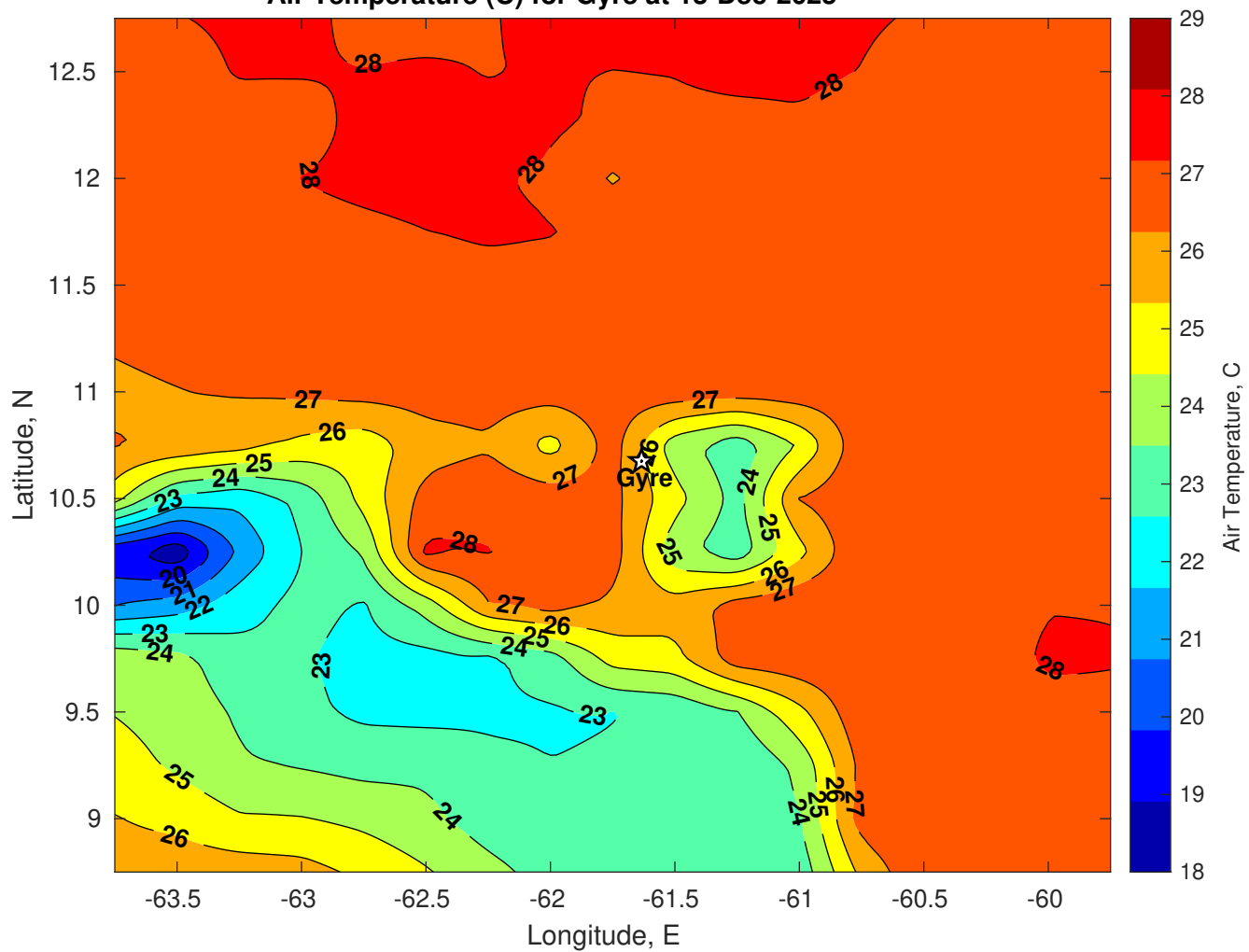
Air Temperature (C) for Gyre at 13-Dec-2025
