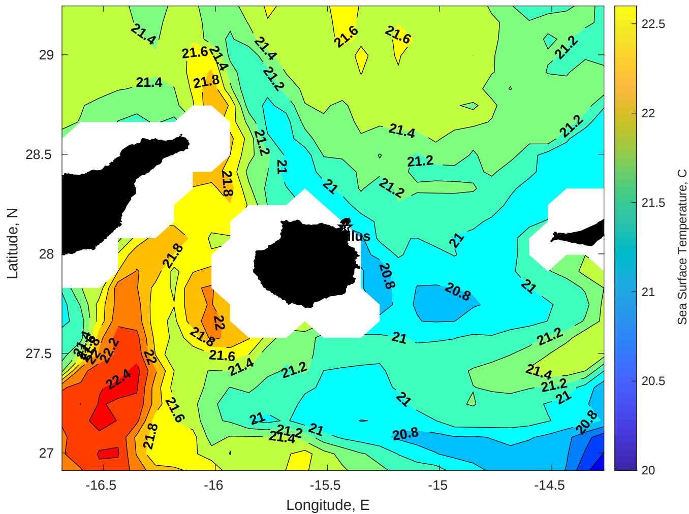
SST for Nautilus at 12-Dec-2025 00:00:00
