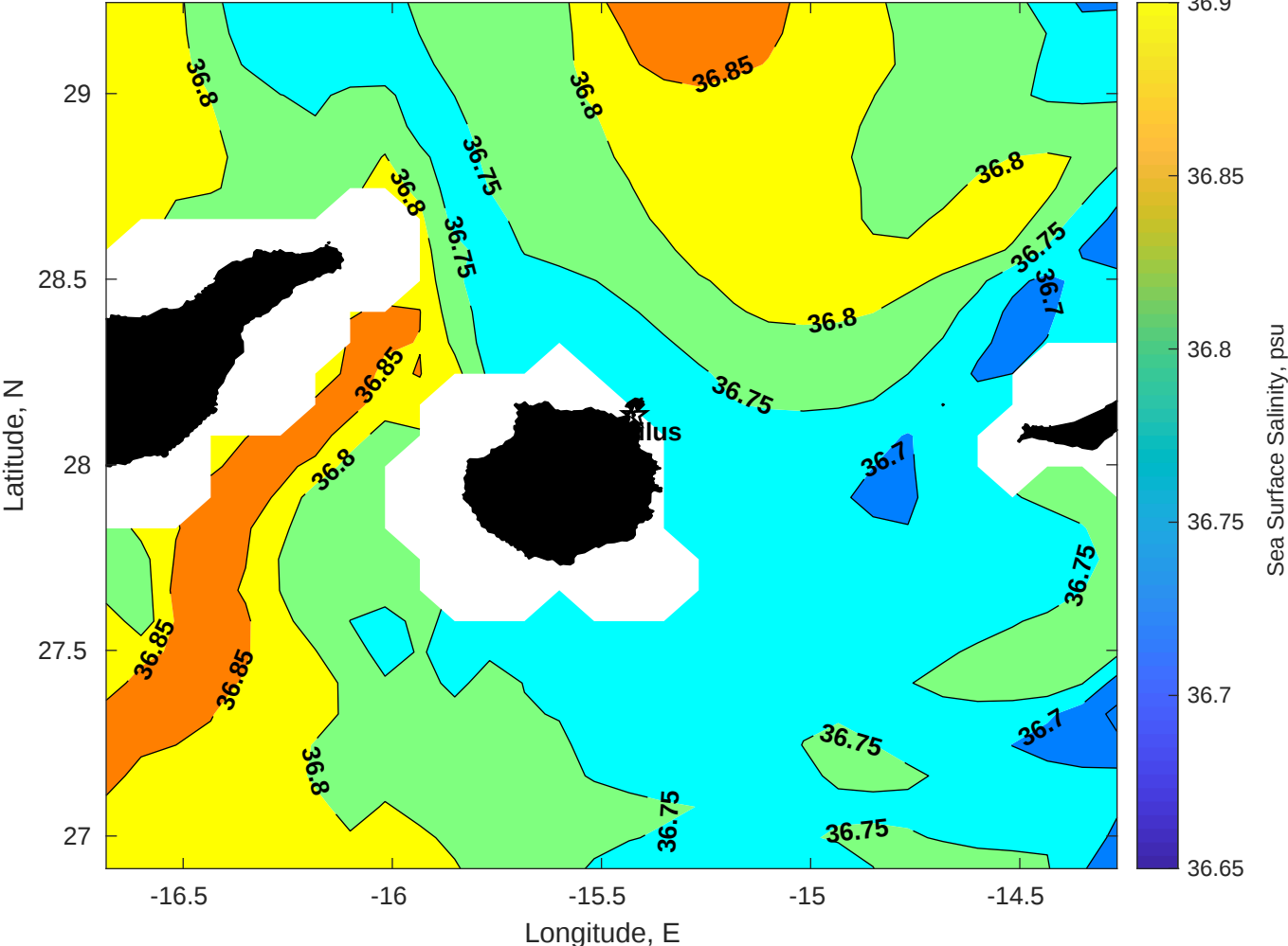
Surface Salinity for Nautilus at 12-Dec-2025 00:00:00
