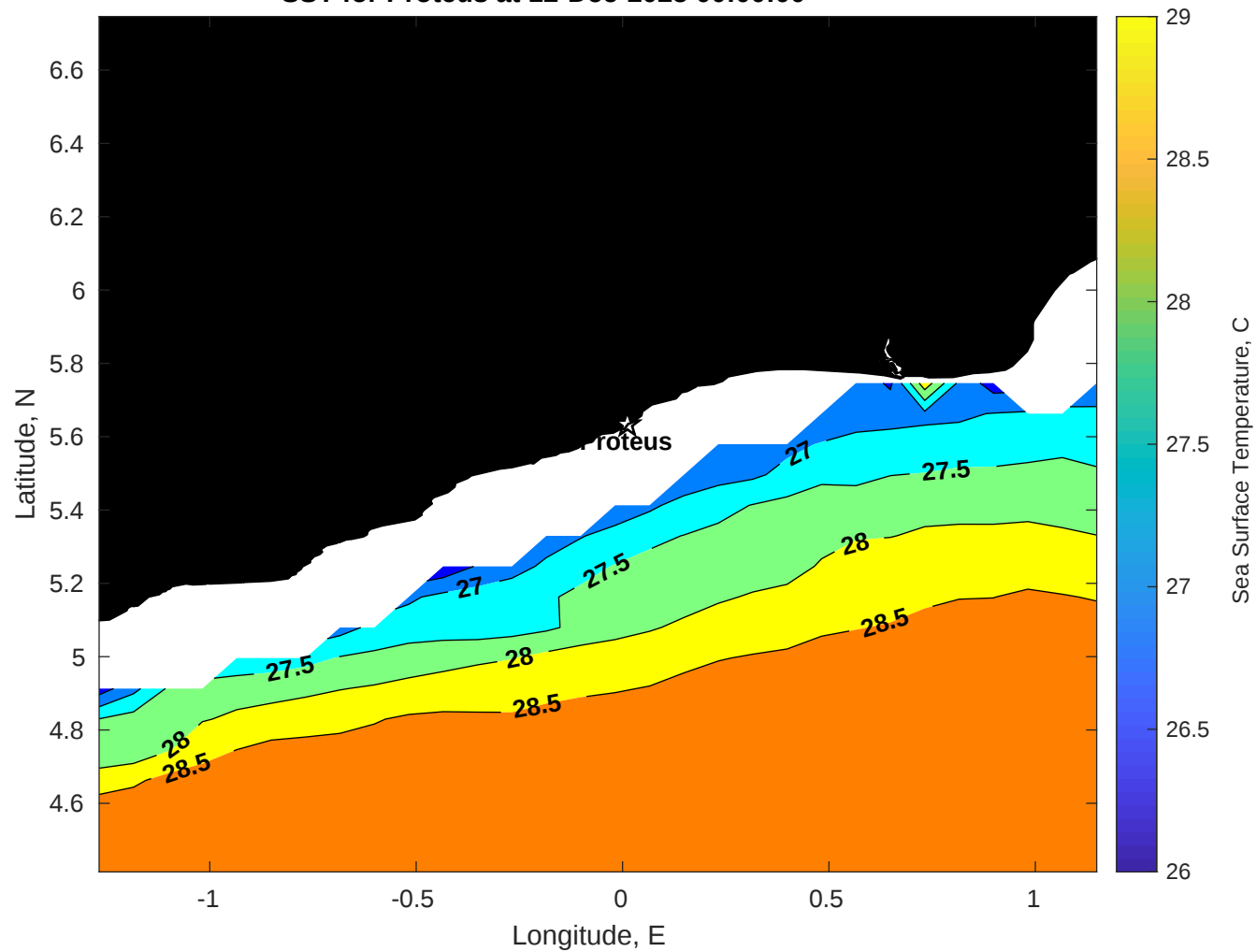
SST for Proteus at 12-Dec-2025 00:00:00
