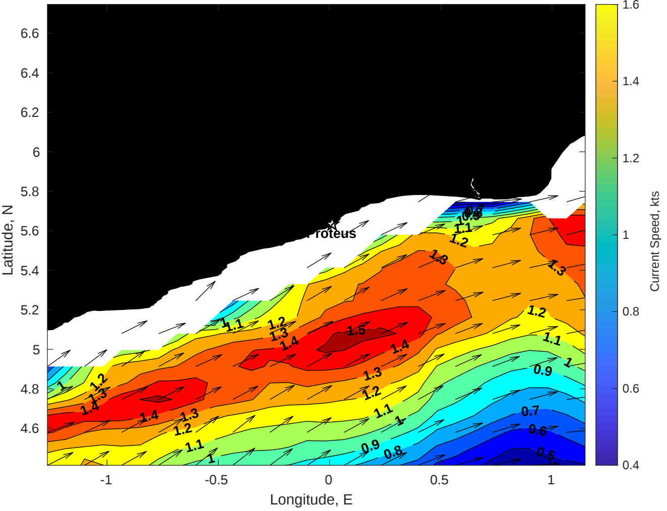
Surface Currents for Proteus at 12-Dec-2025 00:00:00
