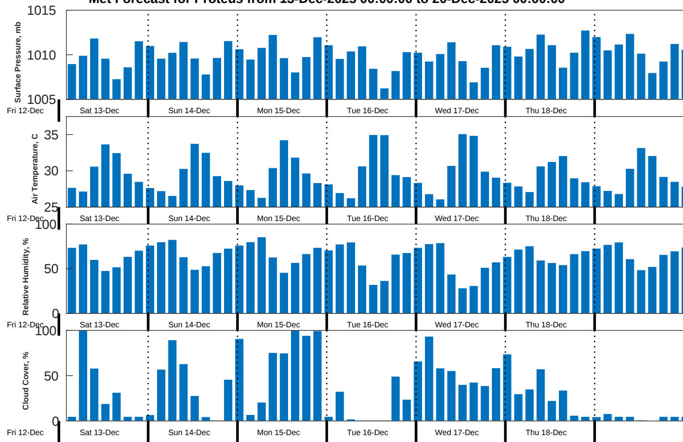
Met Forecast for Proteus from 13-Dec-2025 00:00:00 to 20-Dec-2025 00:00:00
