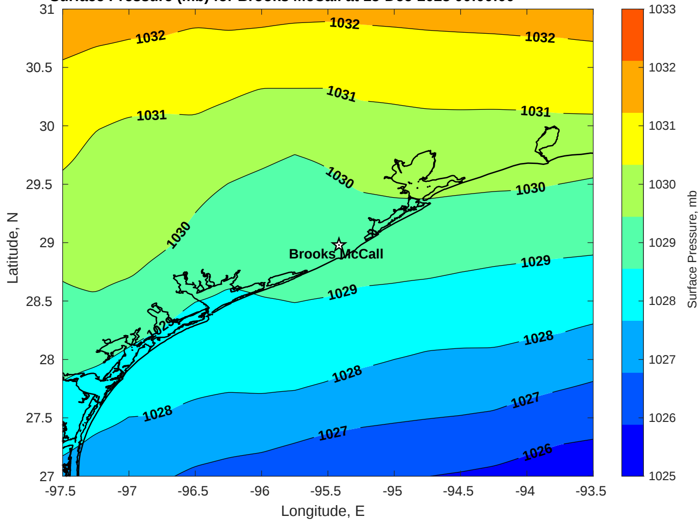
Surface Pressure (mb) for Brooks McCall at 15-Dec-2025 00:00:00
