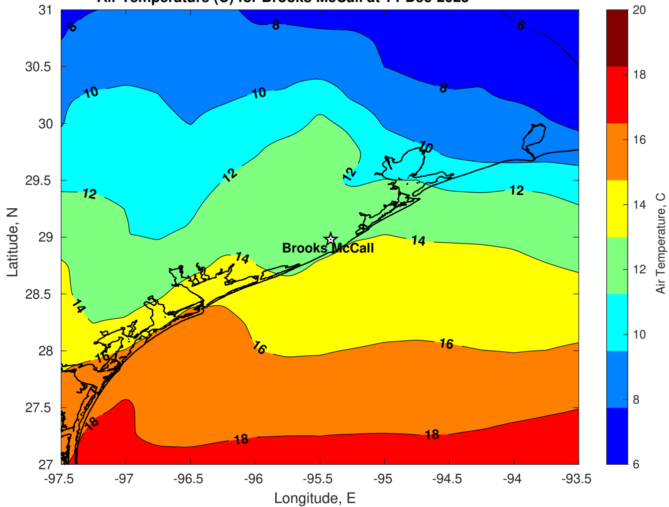
Air Temperature (C) for Brooks McCall at 14-Dec-2025
