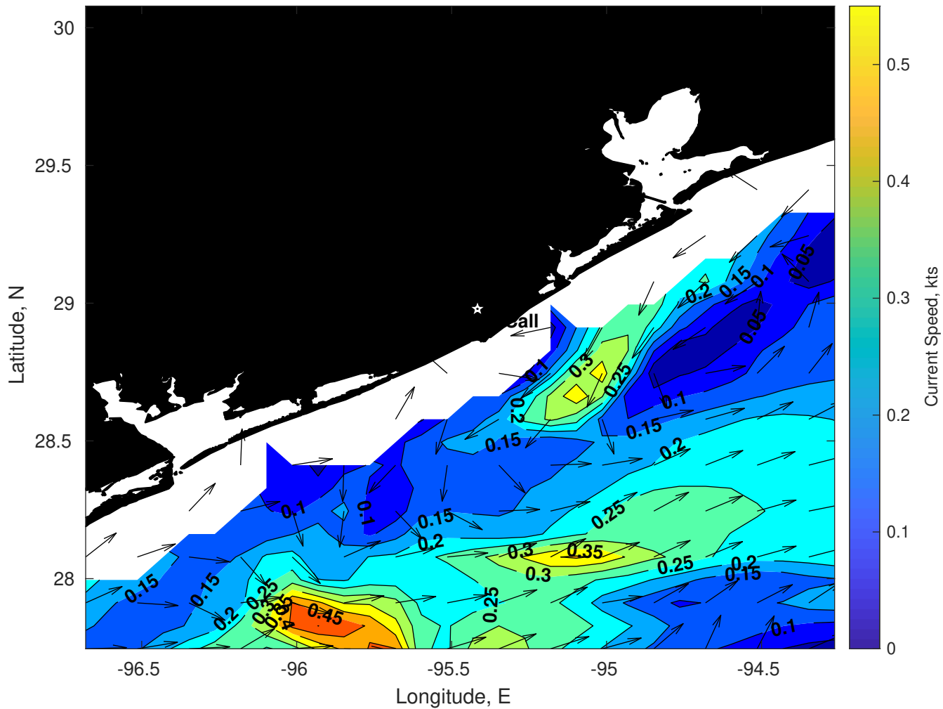
Surface Currents for Brooks McCall at 13-Dec-2025 00:00:00
