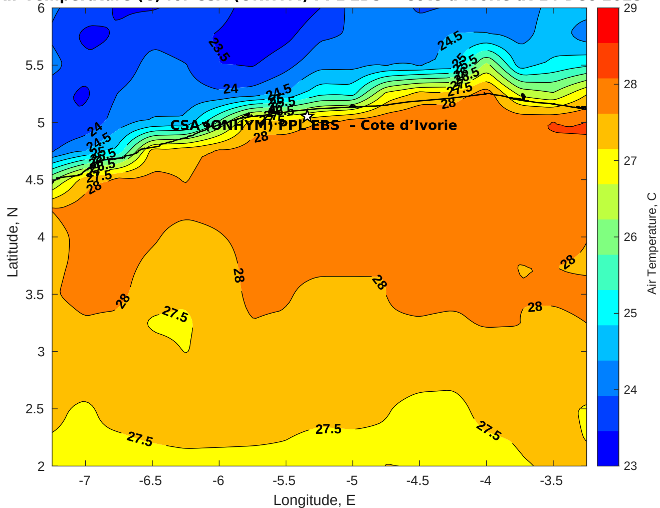
Air Temperature (C) for CSA (ONHYM) PPL EBS - Cote d'Ivoire at 14-Dec-2025
