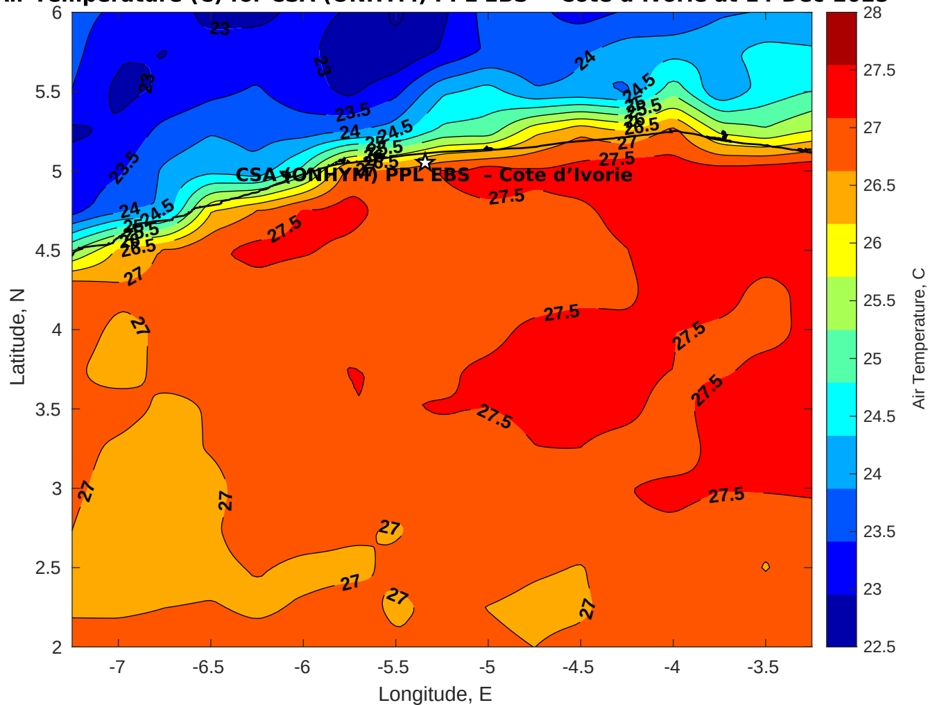
Air Temperature (C) for CSA (ONHYM) PPL EBS - Cote d'Ivoire at 14-Dec-2025
