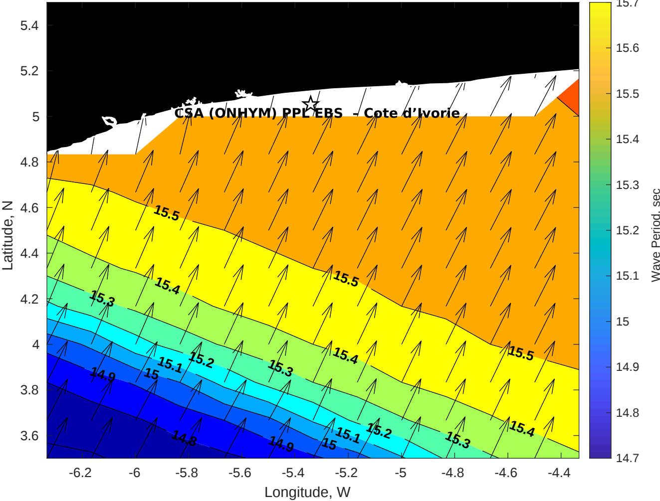
GFS Wave Period (sec) for CSA (ONHYM) PPL EBS - Cote d'Ivoire at 14-Dec-2025 09:00:00
