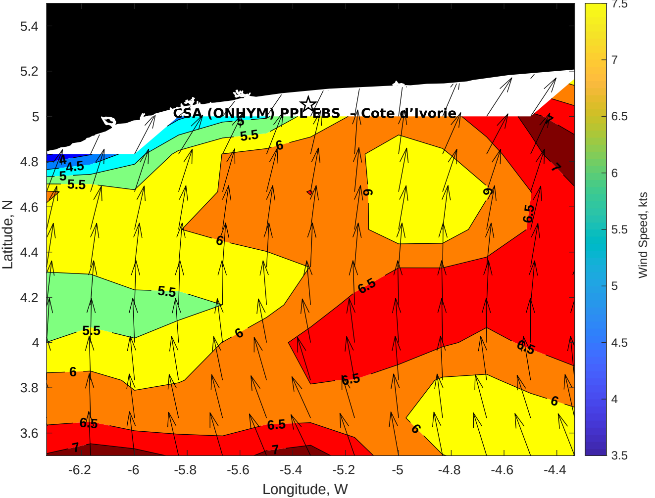
GFS Winds (kts) for CSA (ONHYM) PPL EBS - Cote d'Ivoire at 14-Dec-2025 09:00:00
