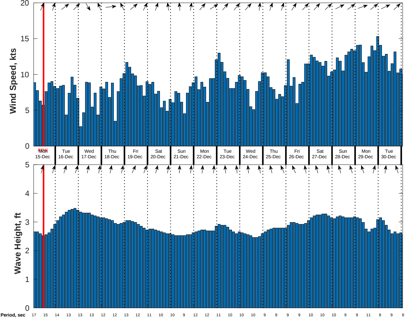
Wind & Wave Forecast for CSA (ONHYM) PPL EBS - Cote d'Ivoire from 14-Dec-2025 01:00:00 to 30-Dec-2025 01:00:00
