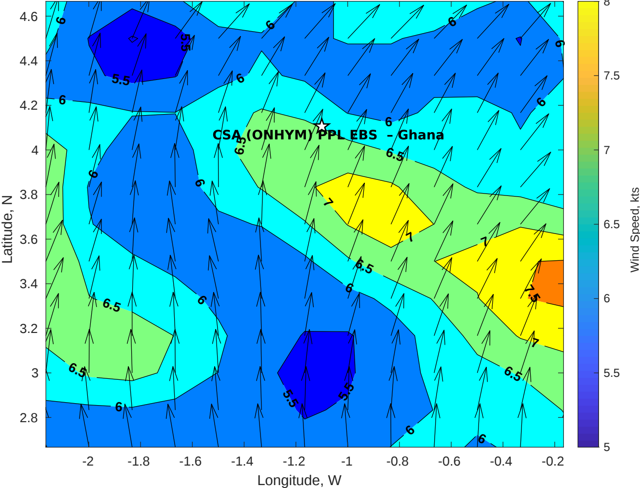
GFS Winds (kts) for CSA (ONHYM) PPL EBS - Ghana at 14-Dec-2025 09:00:00
