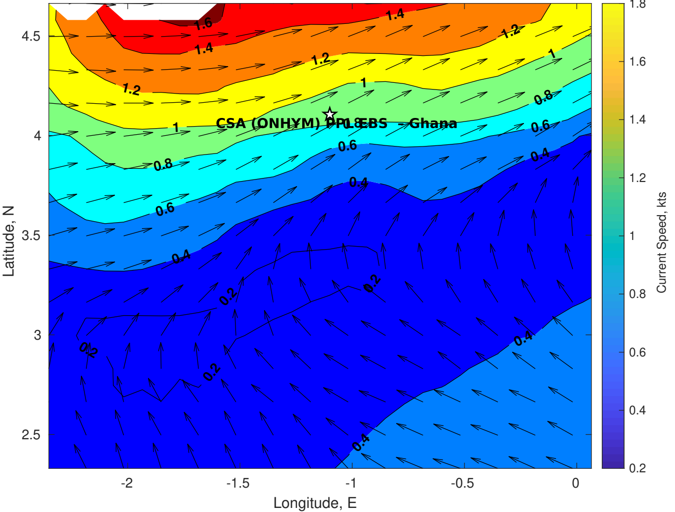
Surface Currents for CSA (ONHYM) PPL EBS - Ghana at 13-Dec-2025 00:00:00
