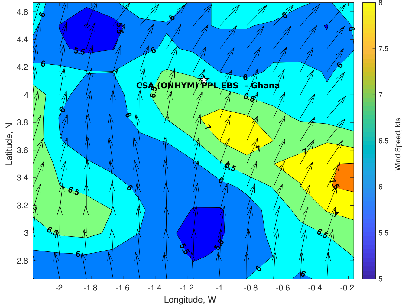
GFS Winds (kts) for CSA (ONHYM) PPL EBS - Ghana at 14-Dec-2025 09:00:00
