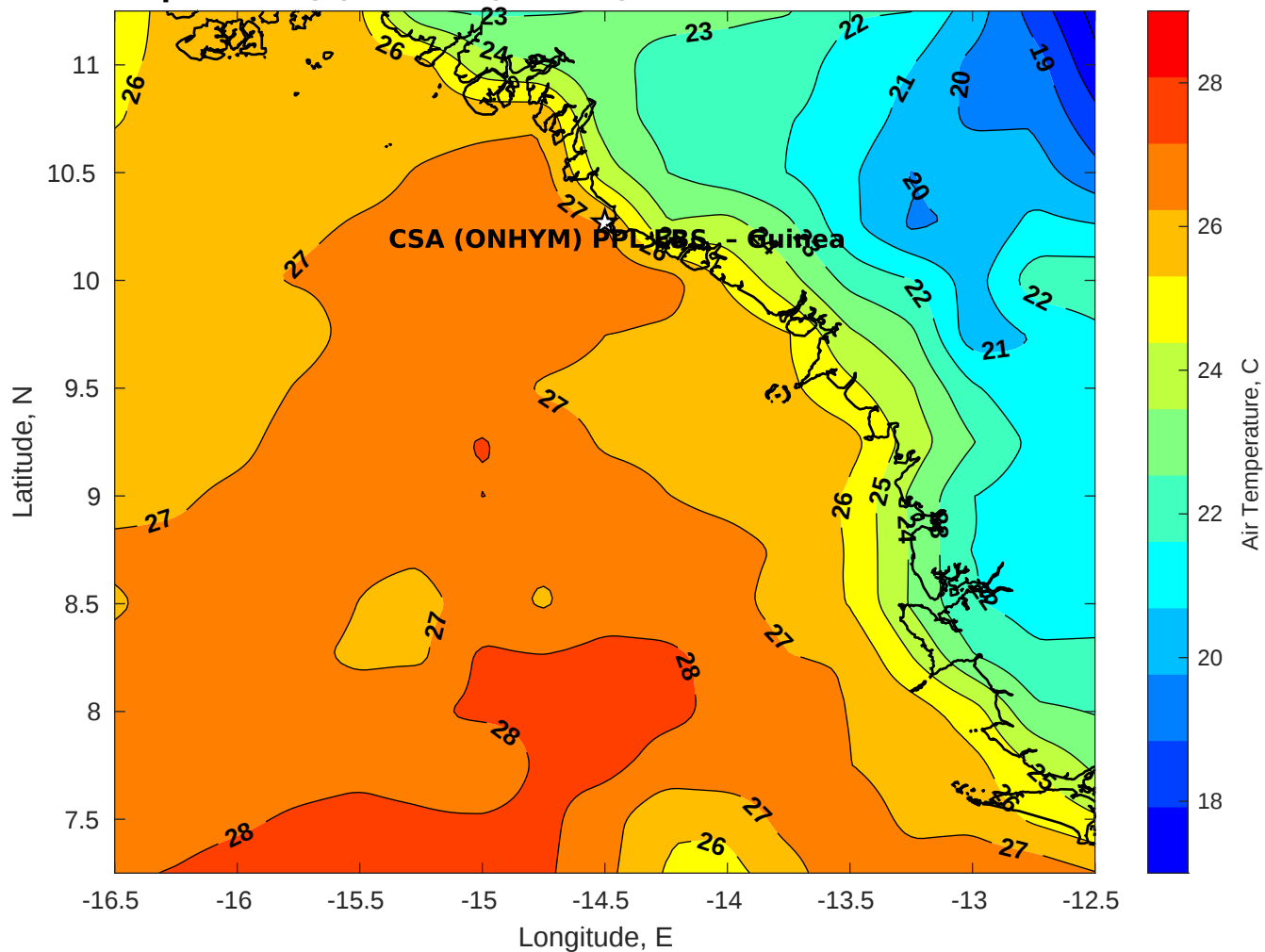
Air Temperature (C) for CSA (ONHYM) PPL EBS - Guinea at 14-Dec-2025
