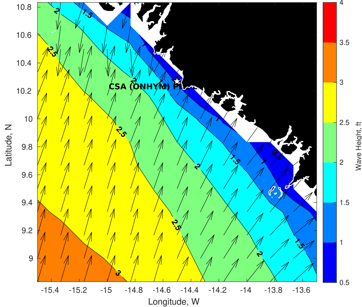
GFS Wave Height (ft) for CSA (ONHYM) PPL EBS - Guinea at 14-Dec-2025 09:00:00
