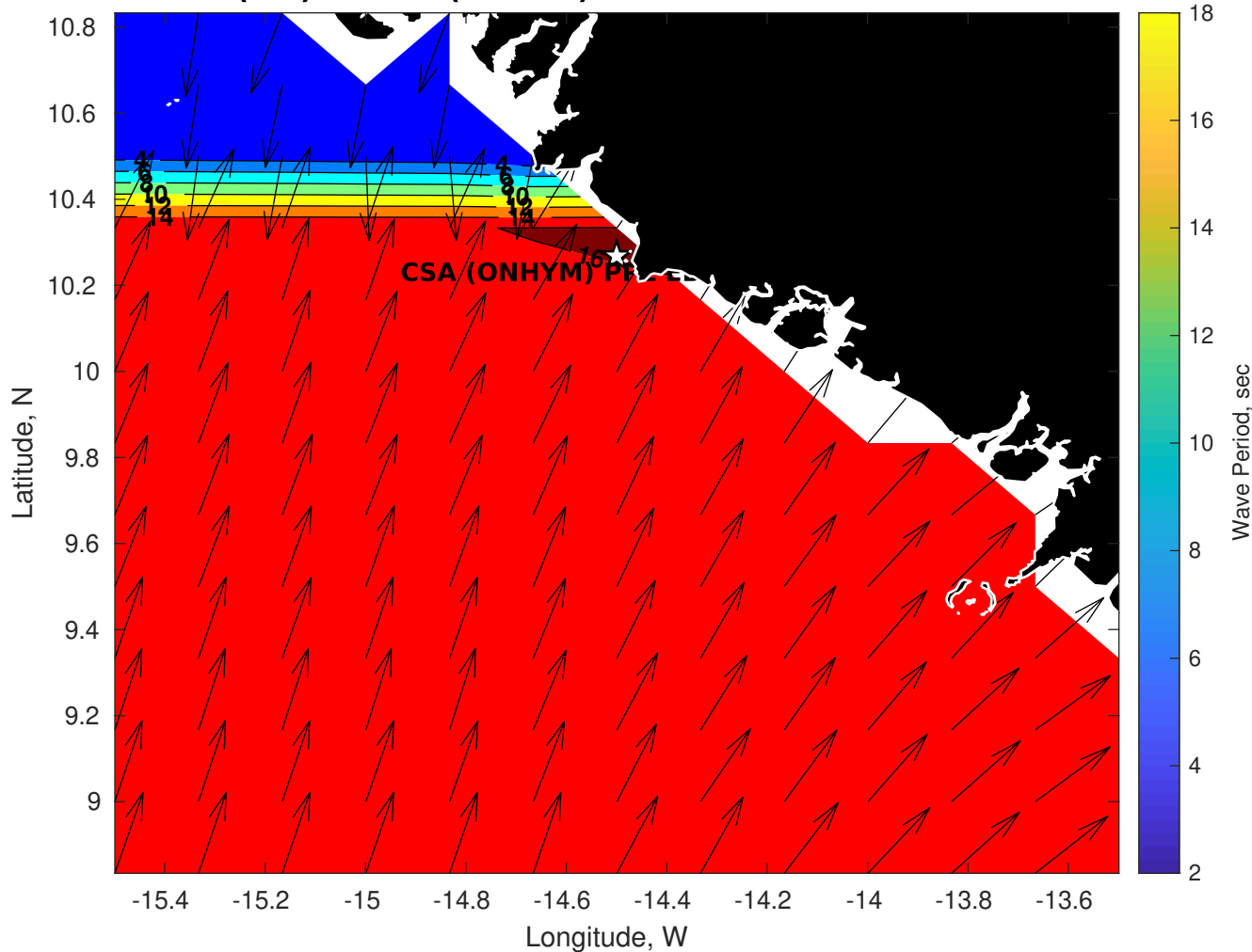
GFS Wave Period (sec) for CSA (ONHYM) PPL EBS - Guinea at 14-Dec-2025 09:00:00
