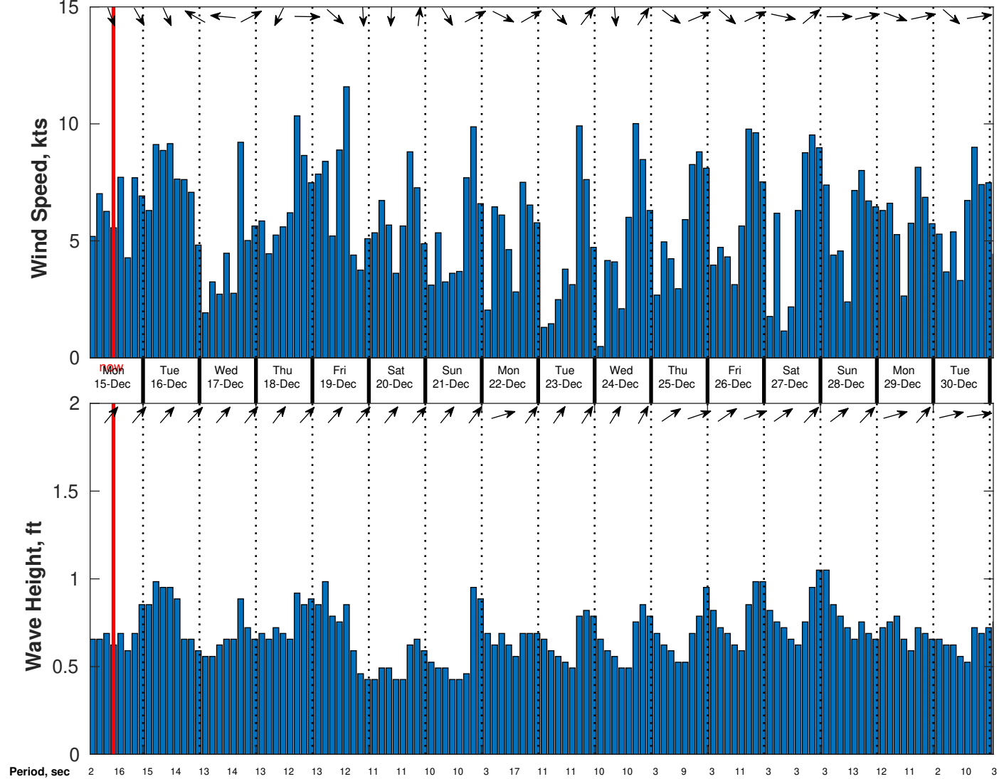
Wind & Wave Forecast for CSA (ONHYM) PPL EBS - Guinea from 14-Dec-2025 01:00:00 to 30-Dec-2025 01:00:00
