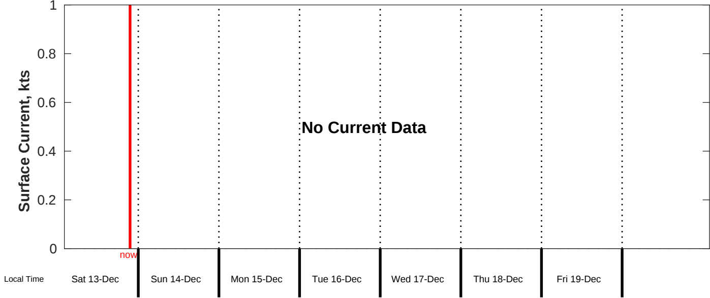
Surface Current Forecast for CSA (ONHYM) PPL EBS - Guinea from 13-Dec-2025 00:00:00 to 21-Dec-2025 00:00:00
