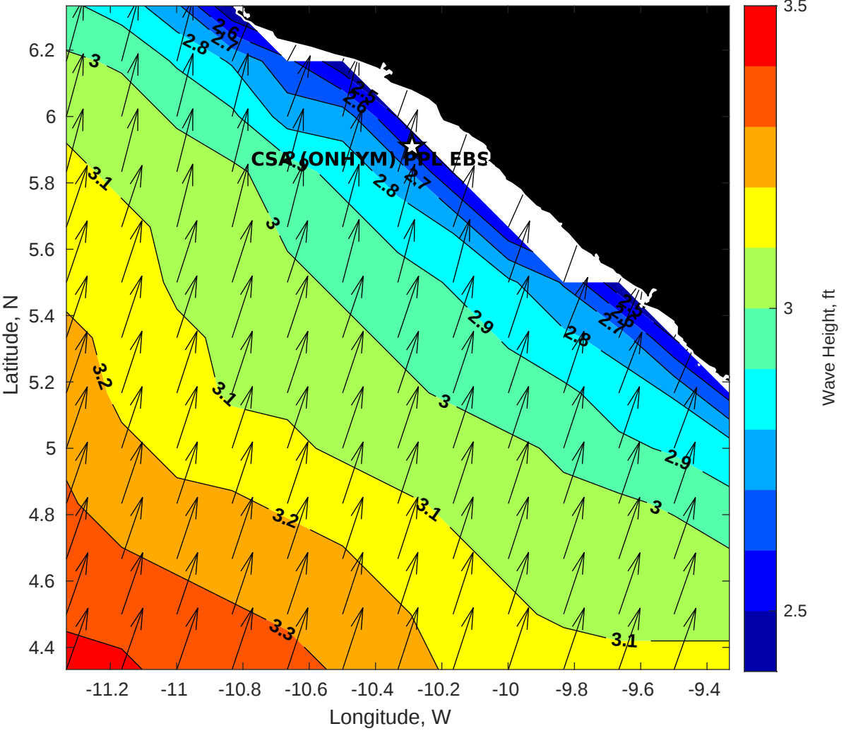
GFS Wave Height (ft) for CSA (ONHYM) PPL EBS - Liberia at 14-Dec-2025 09:00:00
