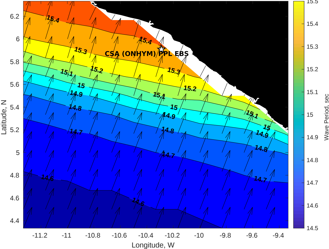
GFS Wave Period (sec) for CSA (ONHYM) PPL EBS - Liberia at 14-Dec-2025 09:00:00
