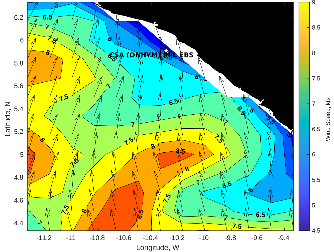
GFS Winds (kts) for CSA (ONHYM) PPL EBS - Liberia at 14-Dec-2025 09:00:00
