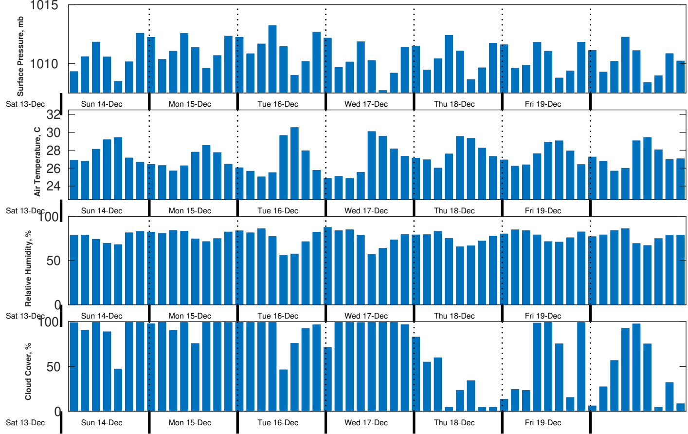
Met Forecast for CSA (ONHYM) PPL EBS - Liberia from 14-Dec-2025 00:00:00 to 21-Dec-2025 00:00:00
