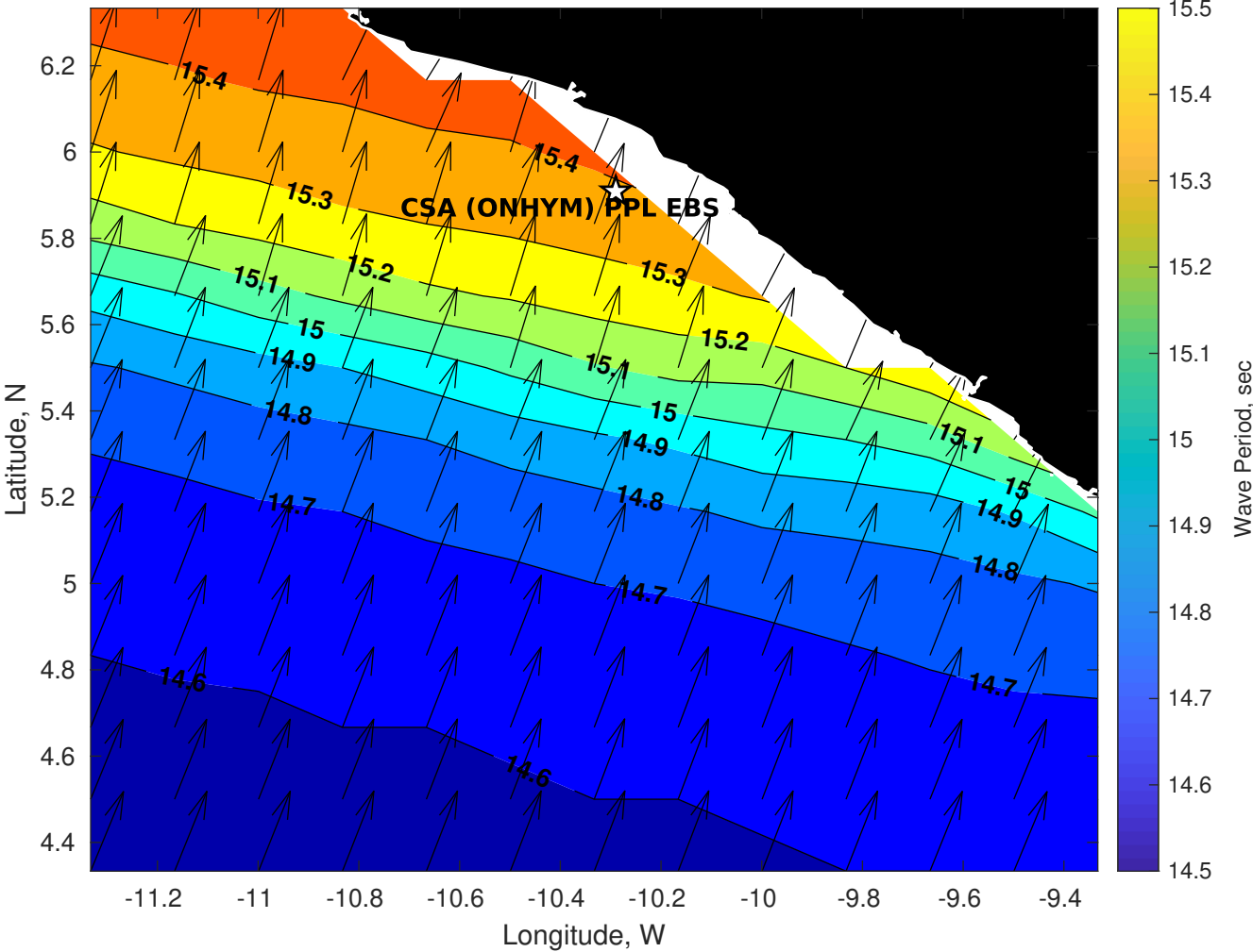
GFS Wave Period (sec) for CSA (ONHYM) PPL EBS - Liberia at 14-Dec-2025 09:00:00
