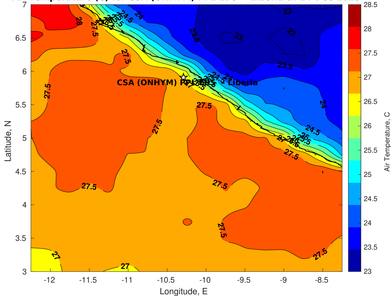
Air Temperature (C) for CSA (ONHYM) PPL EBS - Liberia at 14-Dec-2025
