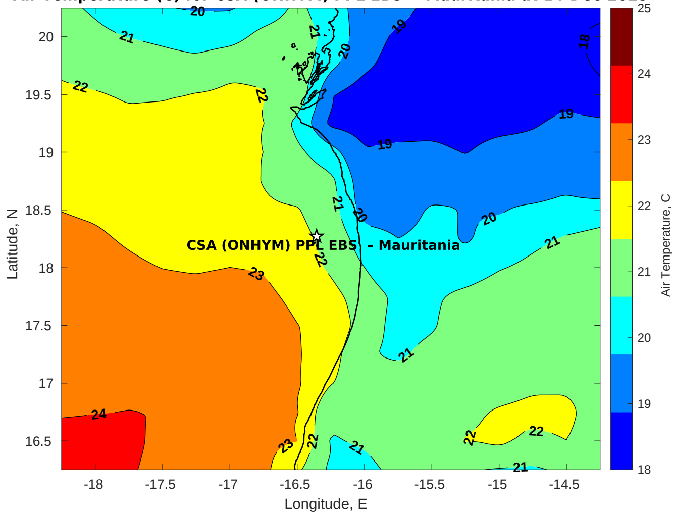
Air Temperature (C) for CSA (ONHYM) PPL EBS - Mauritania at 14-Dec-2025
