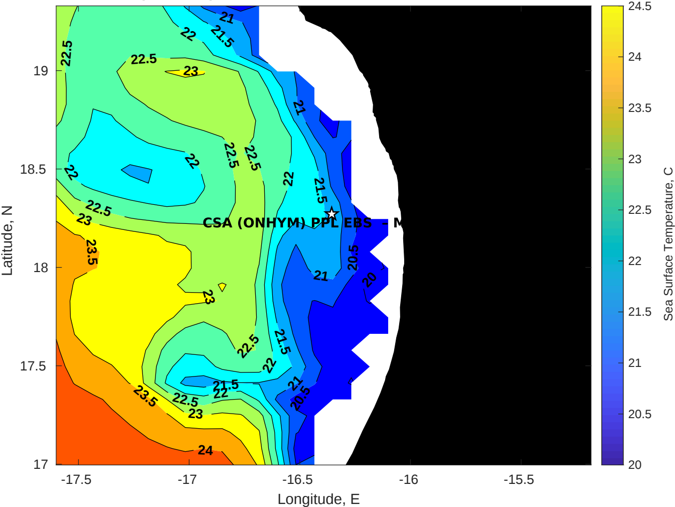
SST for CSA (ONHYM) PPL EBS - Mauritania at 13-Dec-2025 00:00:00
