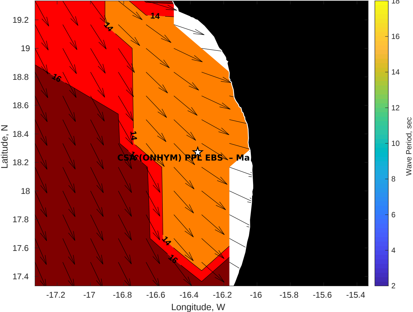
GFS Wave Period (sec) for CSA (ONHYM) PPL EBS - Mauritania at 14-Dec-2025 09:00:00
