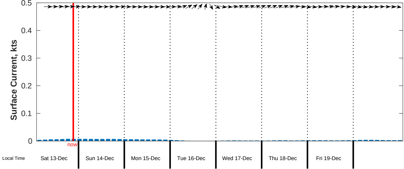
Surface Current Forecast for CSA (ONHYM) PPL EBS - Mauritania from 13-Dec-2025 00:00:00 to 21-Dec-2025 00:00:00
