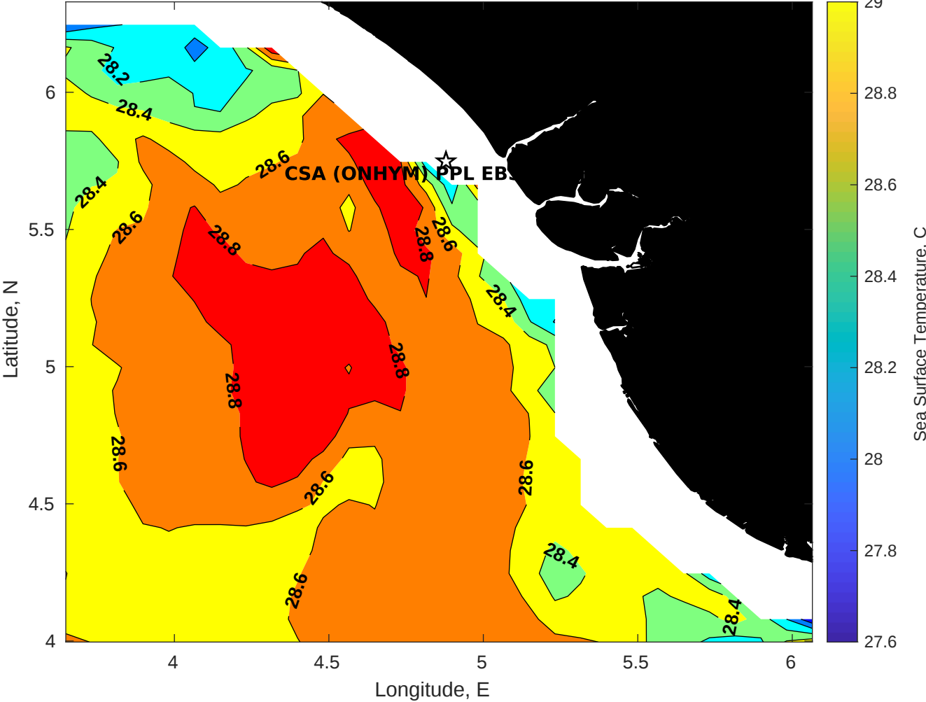
SST for CSA (ONHYM) PPL EBS - Nigeria at 13-Dec-2025 00:00:00
