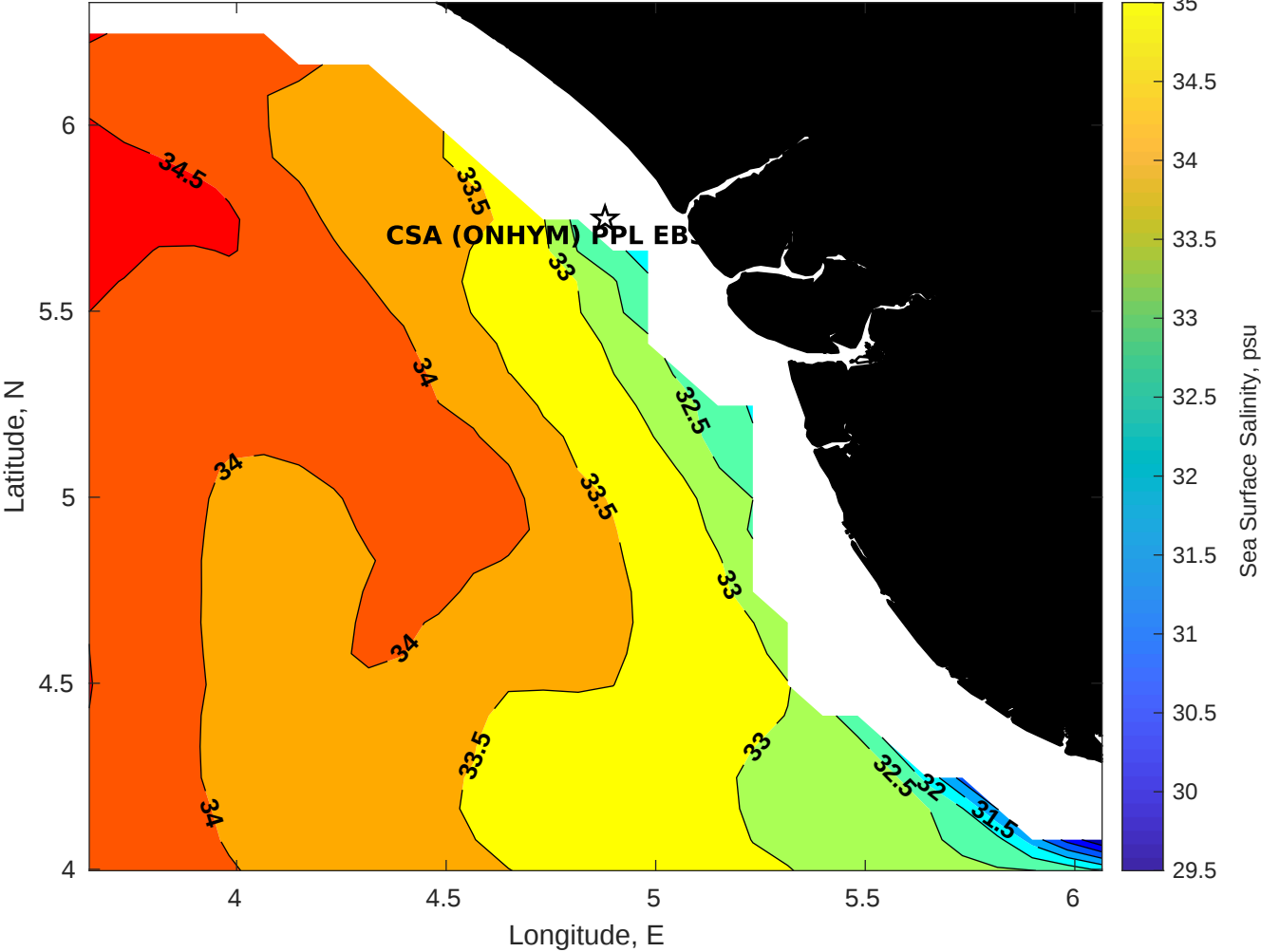
Surface Salinity for CSA (ONHYM) PPL EBS - Nigeria at 13-Dec-2025 00:00:00
