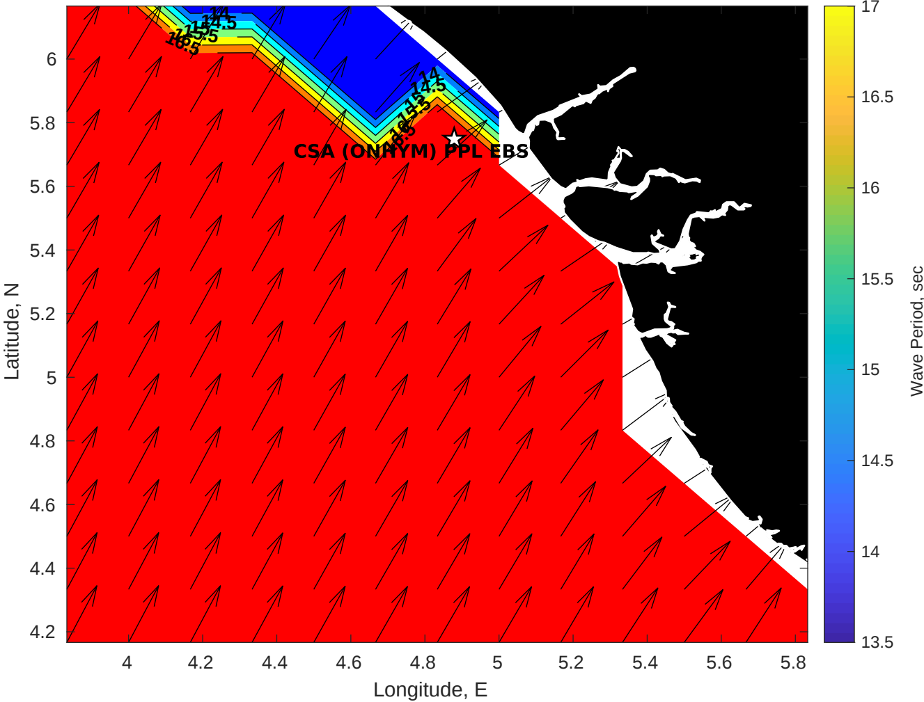
GFS Wave Period (sec) for CSA (ONHYM) PPL EBS - Nigeria at 14-Dec-2025 09:00:00
