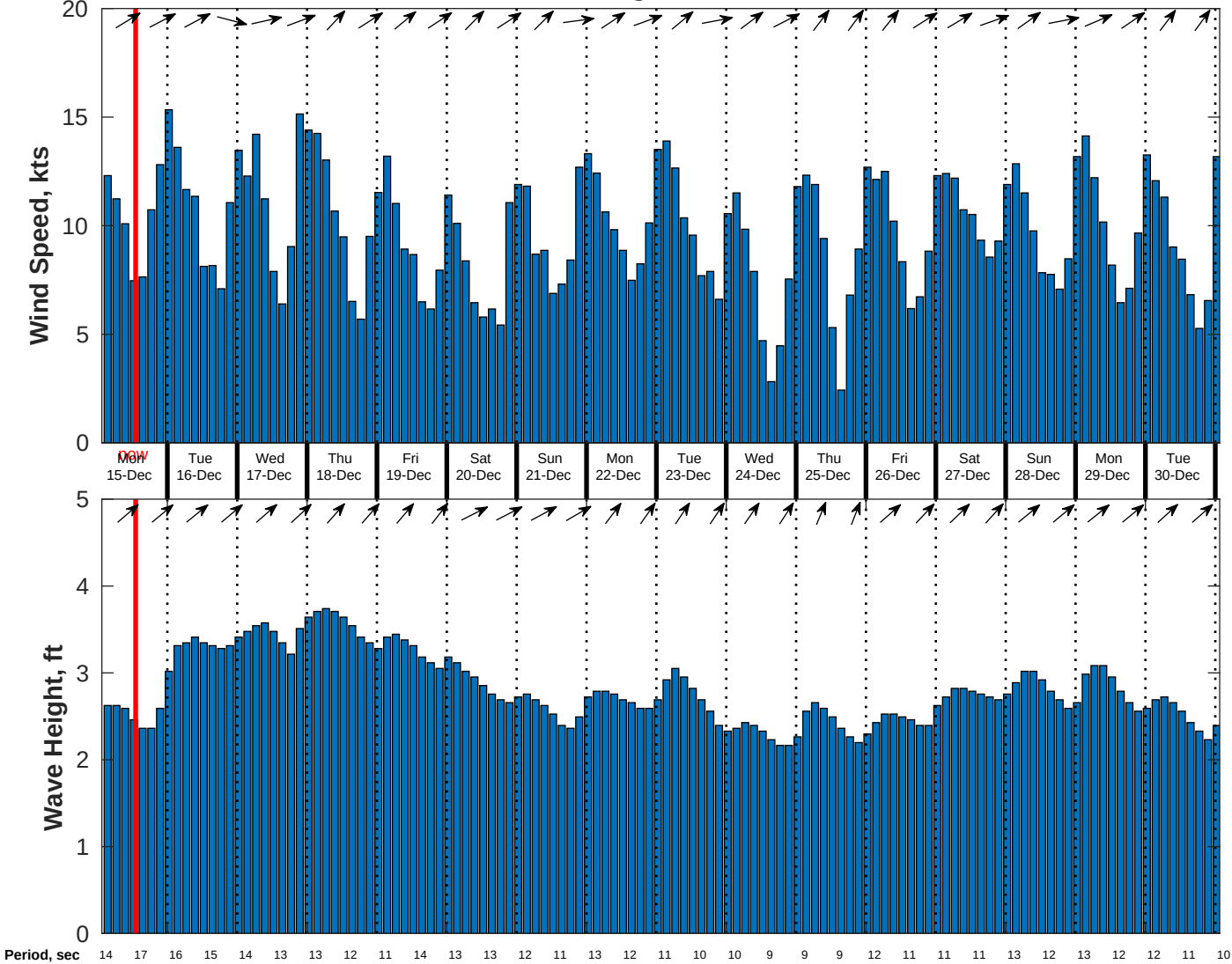
Wind & Wave Forecast for CSA (ONHYM) PPL EBS - Nigeria from 14-Dec-2025 02:00:00 to 30-Dec-2025 02:00:00
