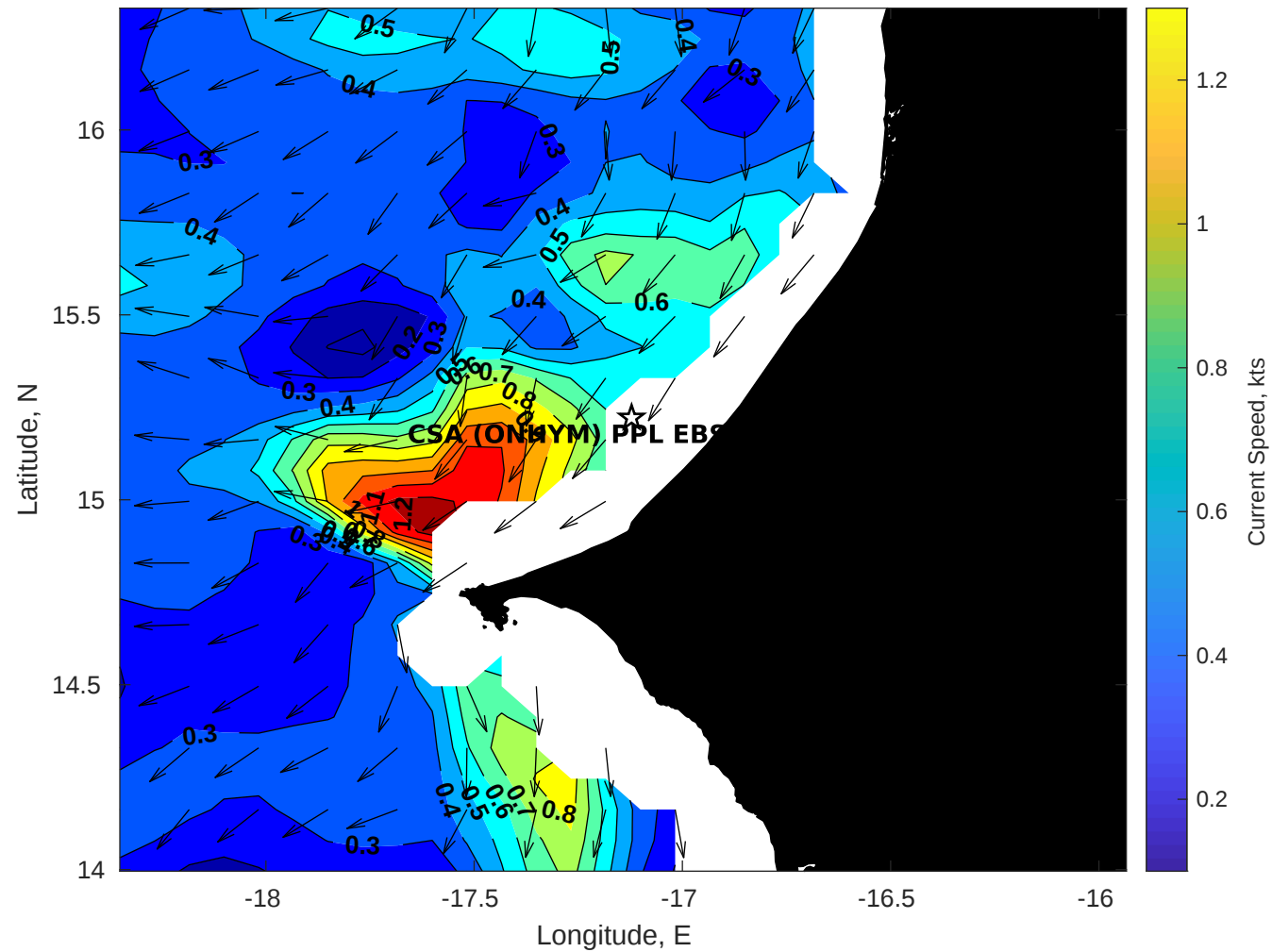
Surface Currents for CSA (ONHYM) PPL EBS - Senegal at 13-Dec-2025 00:00:00
