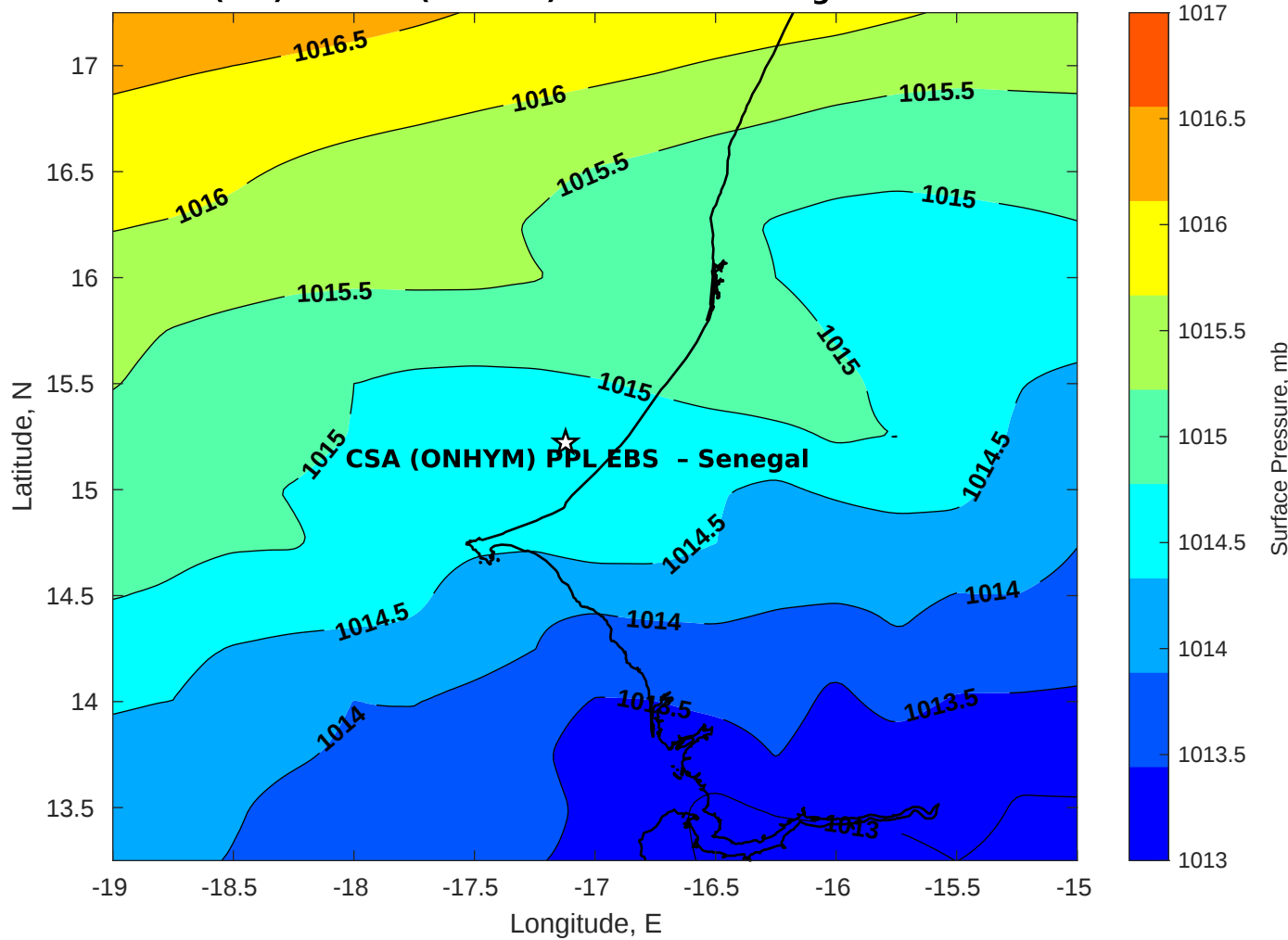
Surface Pressure (mb) for CSA (ONHYM) PPL EBS - Senegal at 16-Dec-2025 00:00:00
