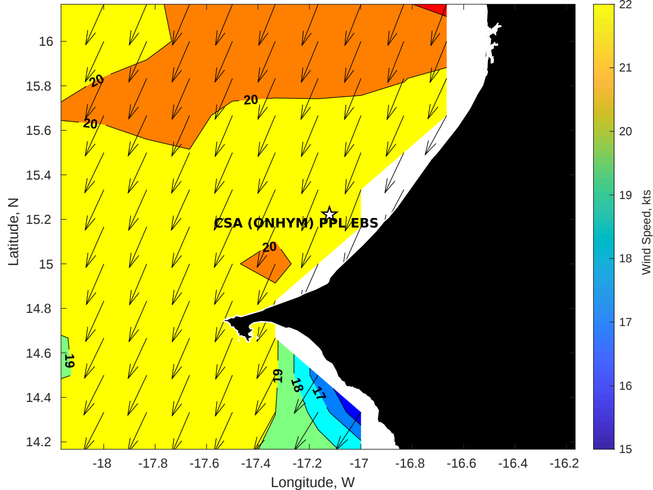
GFS Winds (kts) for CSA (ONHYM) PPL EBS - Senegal at 14-Dec-2025 09:00:00
