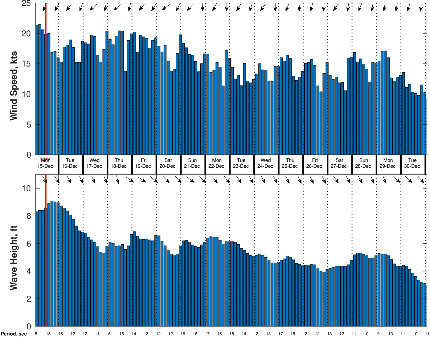
Wind & Wave Forecast for CSA (ONHYM) PPL EBS - Senegal from 14-Dec-2025 01:00:00 to 30-Dec-2025 01:00:00
