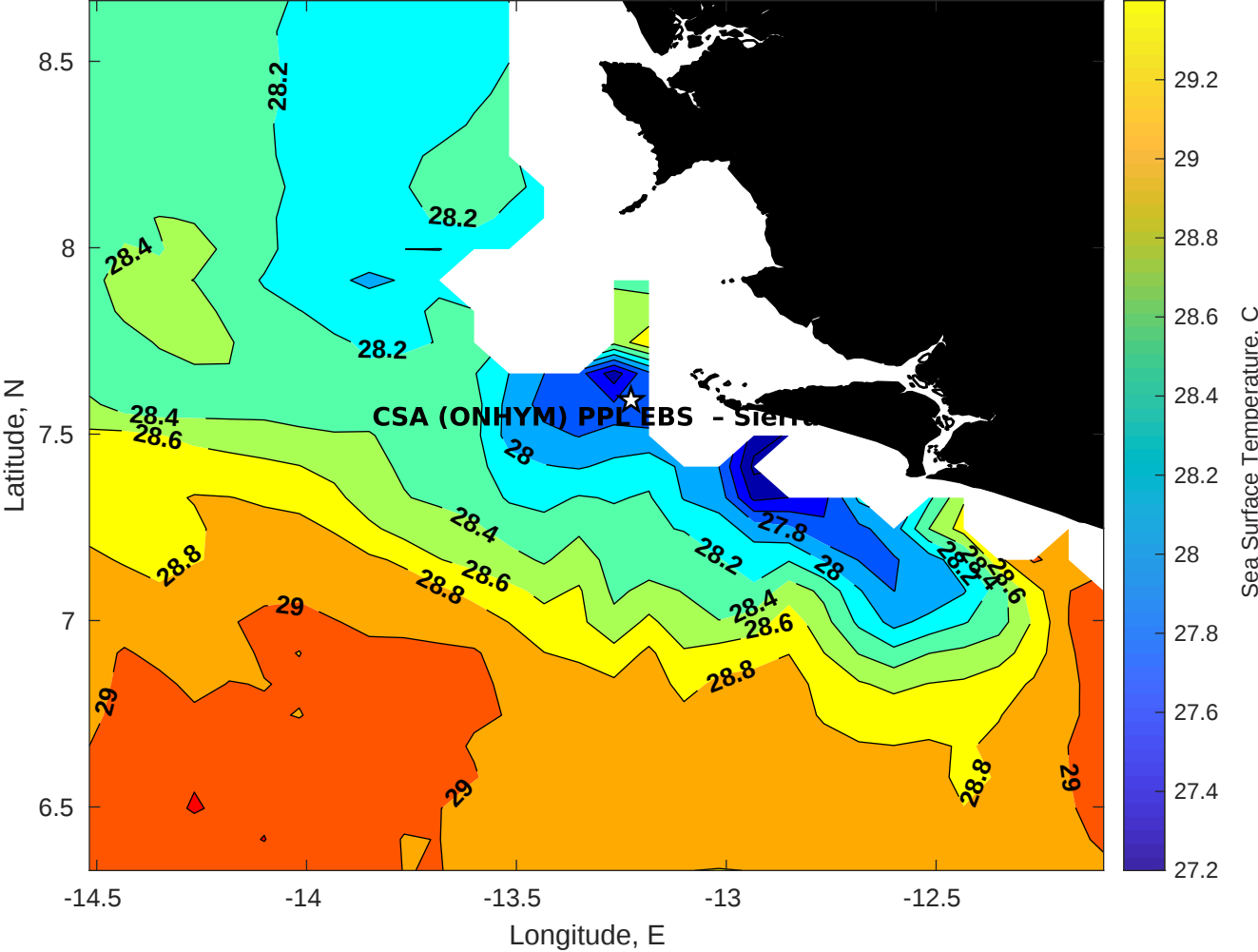
SST for CSA (ONHYM) PPL EBS - Sierra Leone at 13-Dec-2025 00:00:00
