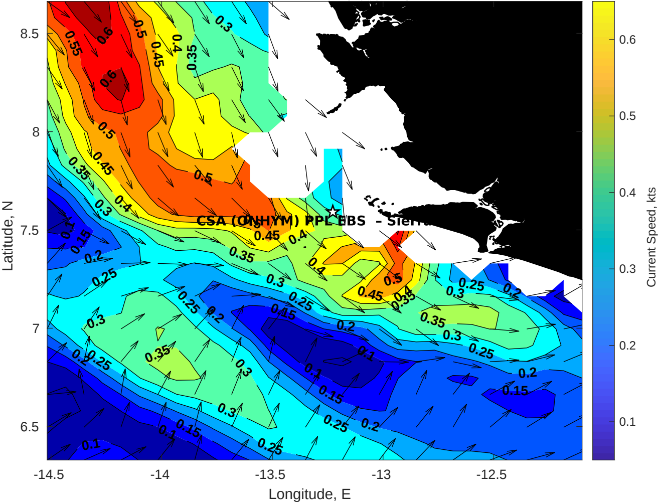
Surface Currents for CSA (ONHYM) PPL EBS - Sierra Leone at 13-Dec-2025 00:00:00
