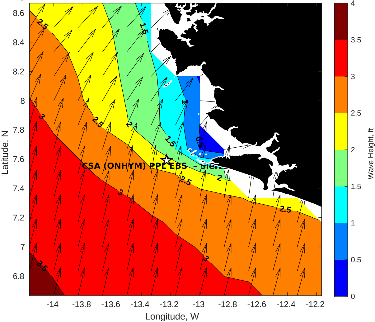
GFS Wave Height (ft) for CSA (ONHYM) PPL EBS - Sierra Leone at 14-Dec-2025 09:00:00
